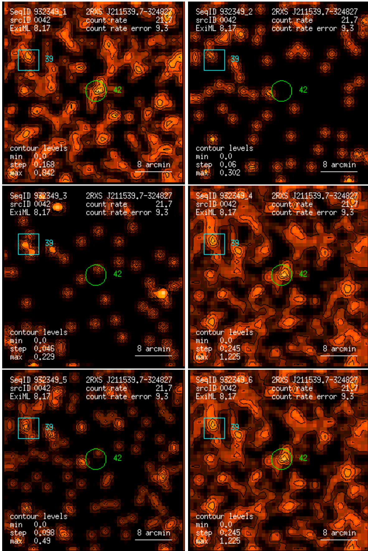
Figure 42: RASS 932349: detection 0042: band rate images, Gaussian filter: (1) PSPC channels 11 – 41, (2) 52 – 90, (3) 91 – 201, (4) 11 – 235, (5) 52 – 201, (6) 11 – 201. Broad band rates in counts/ks. Band rate contour levels in counts/ks/arcmin 2 .
