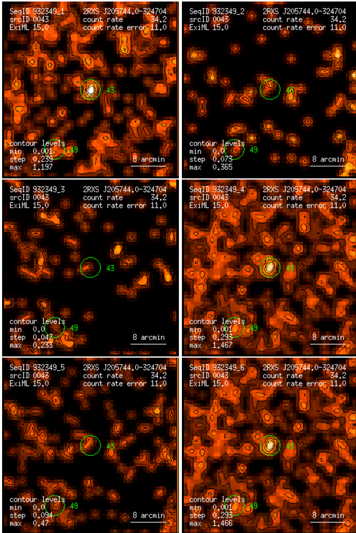
Figure 43: RASS 932349: detection 0043: band rate images, Gaussian filter: (1) PSPC channels 11 – 41, (2) 52 – 90, (3) 91 – 201, (4) 11 – 235, (5) 52 – 201, (6) 11 – 201. Broad band rates in counts/ks. Band rate contour levels in counts/ks/arcmin 2 .
