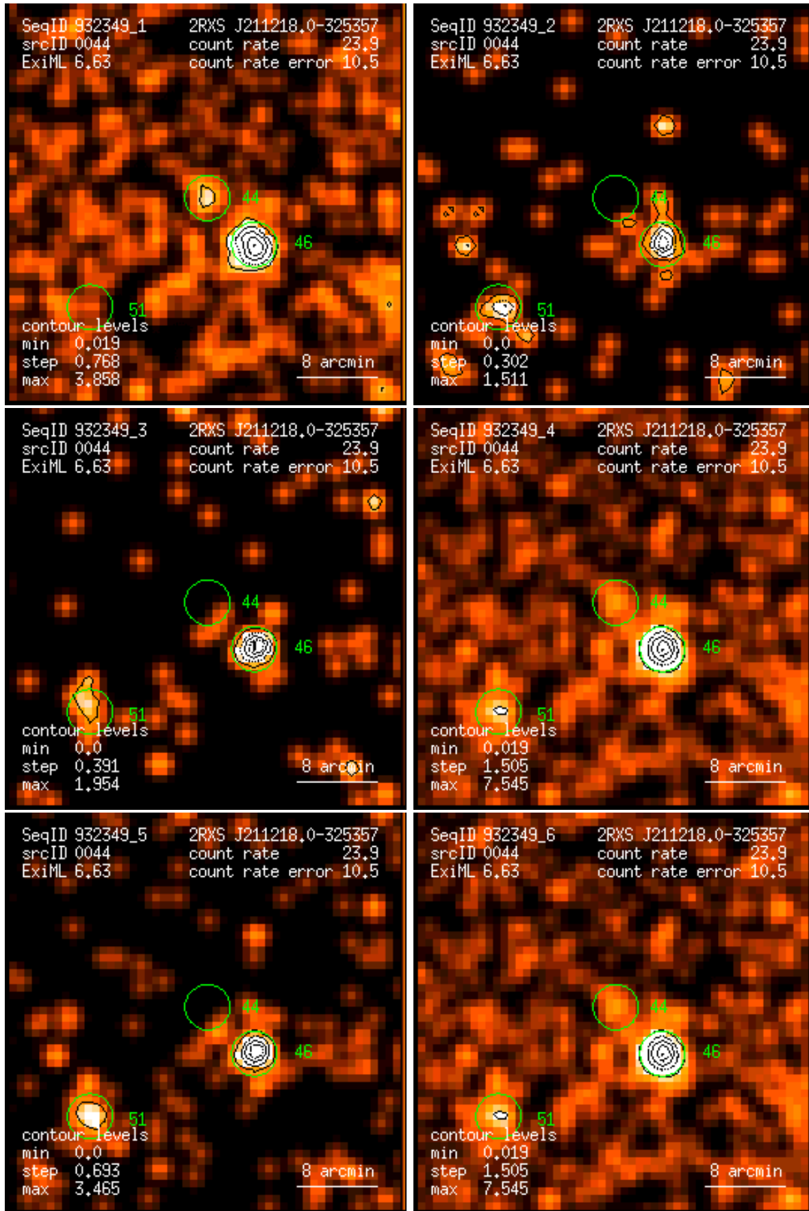
Figure 44: RASS 932349: detection 0044: band rate images, Gaussian filter: (1) PSPC channels 11 – 41, (2) 52 – 90, (3) 91 – 201, (4) 11 – 235, (5) 52 – 201, (6) 11 – 201. Broad band rates in counts/ks. Band rate contour levels in counts/ks/arcmin 2 .
