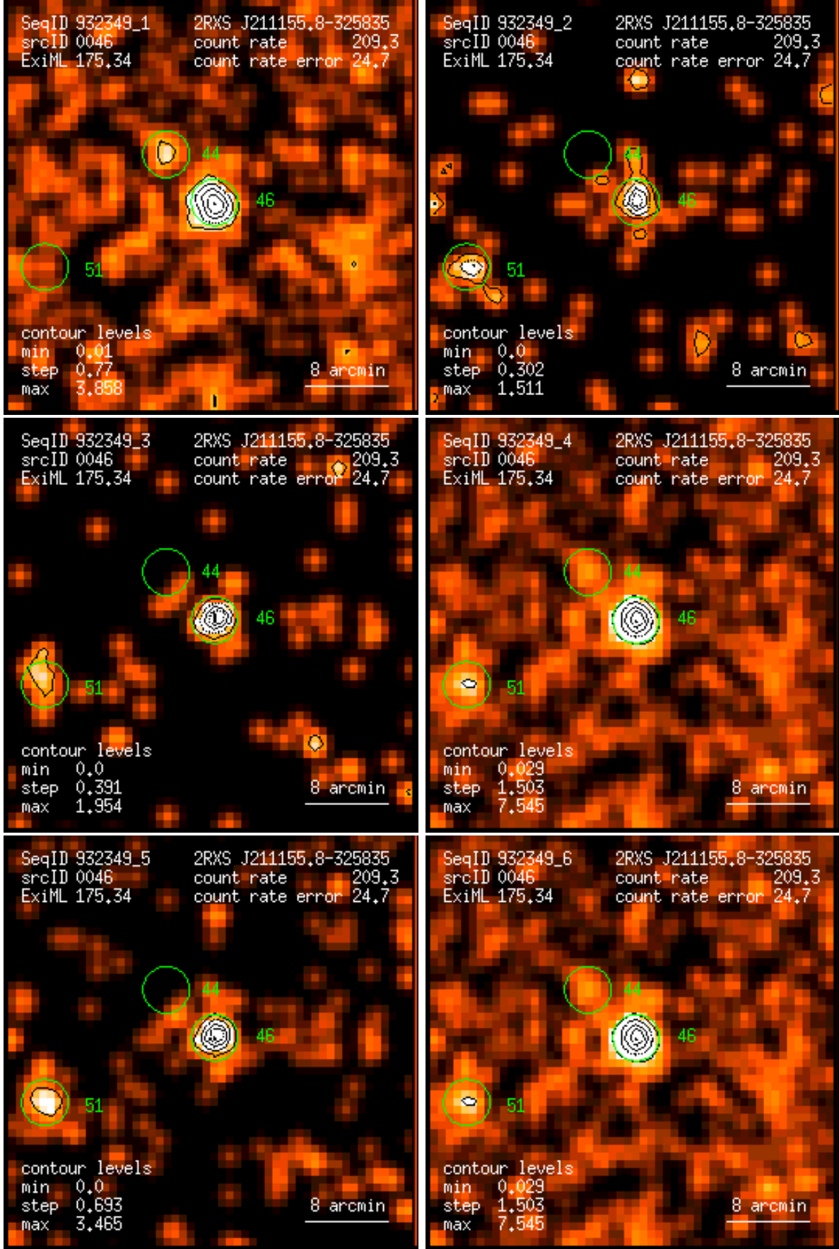
Figure 46: RASS 932349: detection 0046: band rate images, Gaussian filter: (1) PSPC channels 11 – 41, (2) 52 – 90, (3) 91 – 201, (4) 11 – 235, (5) 52 – 201, (6) 11 – 201. Broad band rates in counts/ks. Band rate contour levels in counts/ks/arcmin 2 .
