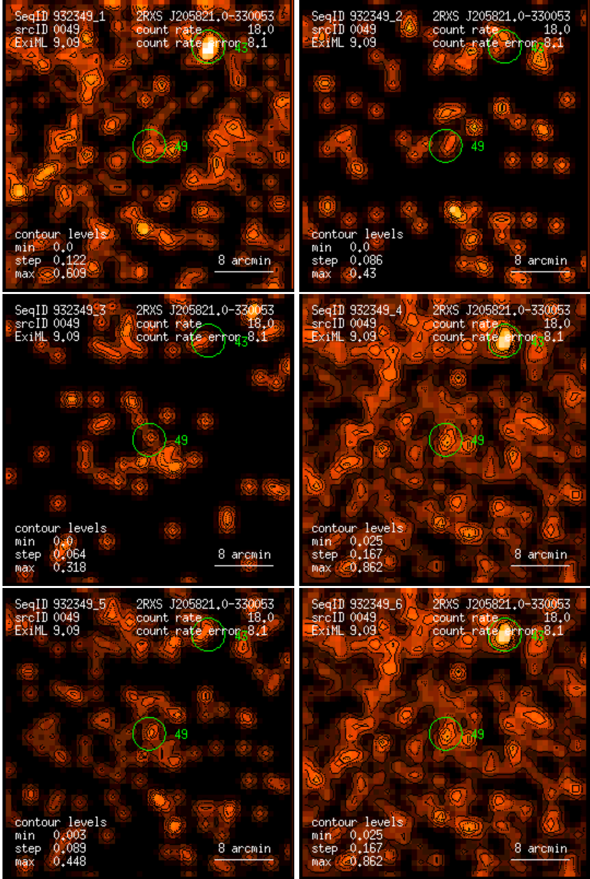
Figure 49: RASS 932349: detection 0049: band rate images, Gaussian filter: (1) PSPC channels 11 – 41, (2) 52 – 90, (3) 91 – 201, (4) 11 – 235, (5) 52 – 201, (6) 11 – 201. Broad band rates in counts/ks. Band rate contour levels in counts/ks/arcmin 2 .
