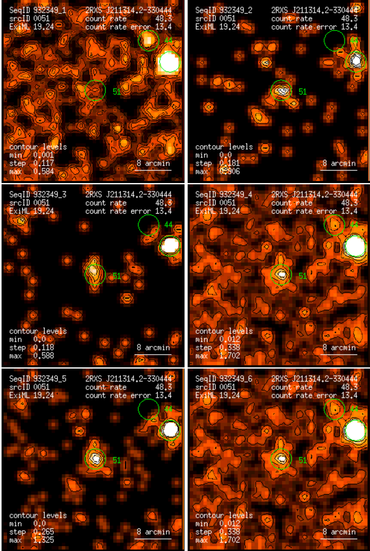
Figure 51: RASS 932349: detection 0051: band rate images, Gaussian filter: (1) PSPC channels 11 – 41, (2) 52 – 90, (3) 91 – 201, (4) 11 – 235, (5) 52 – 201, (6) 11 – 201. Broad band rates in counts/ks. Band rate contour levels in counts/ks/arcmin 2 .
