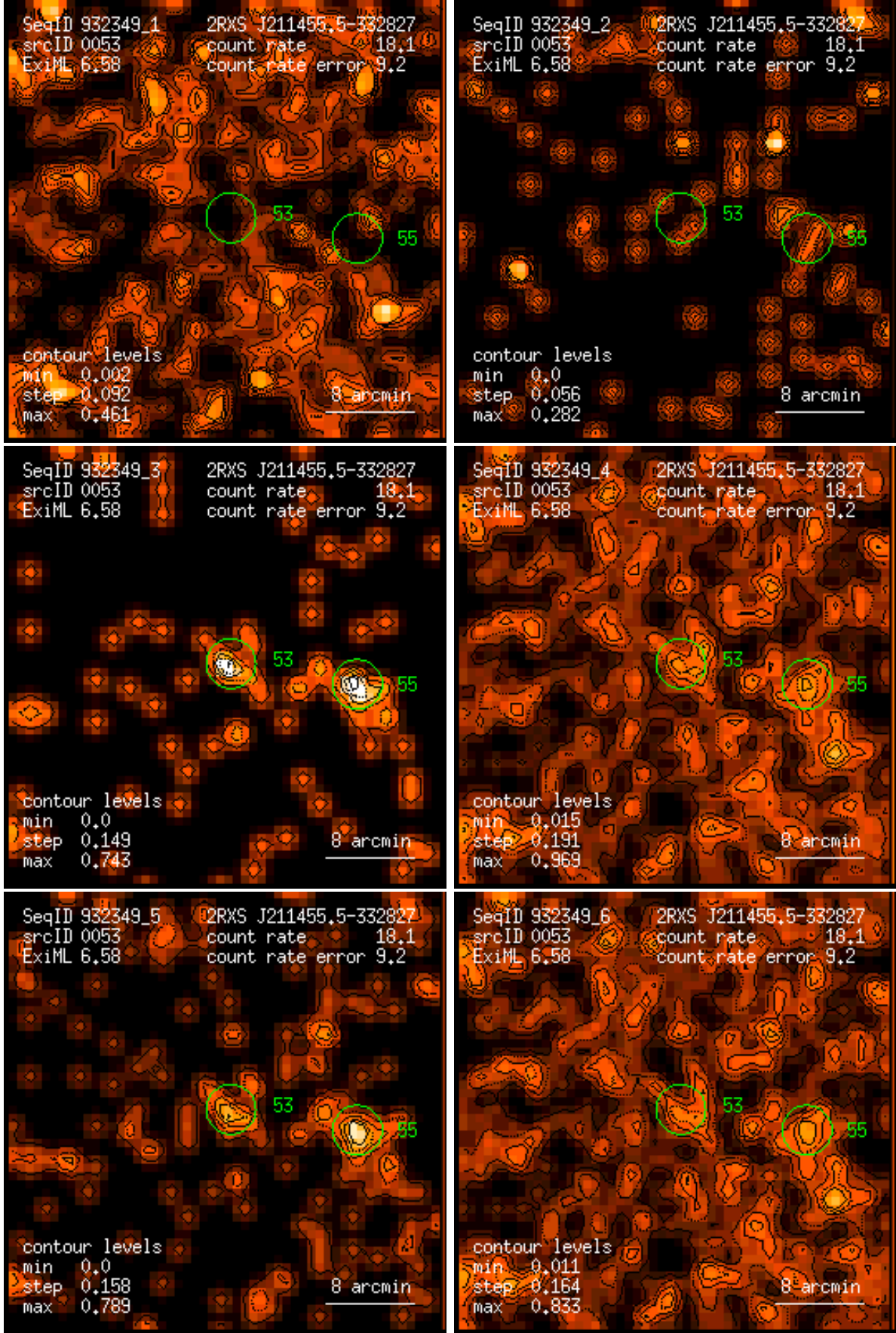
Figure 53: RASS 932349: detection 0053: band rate images, Gaussian filter: (1) PSPC channels 11 – 41, (2) 52 – 90, (3) 91 – 201, (4) 11 – 235, (5) 52 – 201, (6) 11 – 201. Broad band rates in counts/ks. Band rate contour levels in counts/ks/arcmin 2 .
