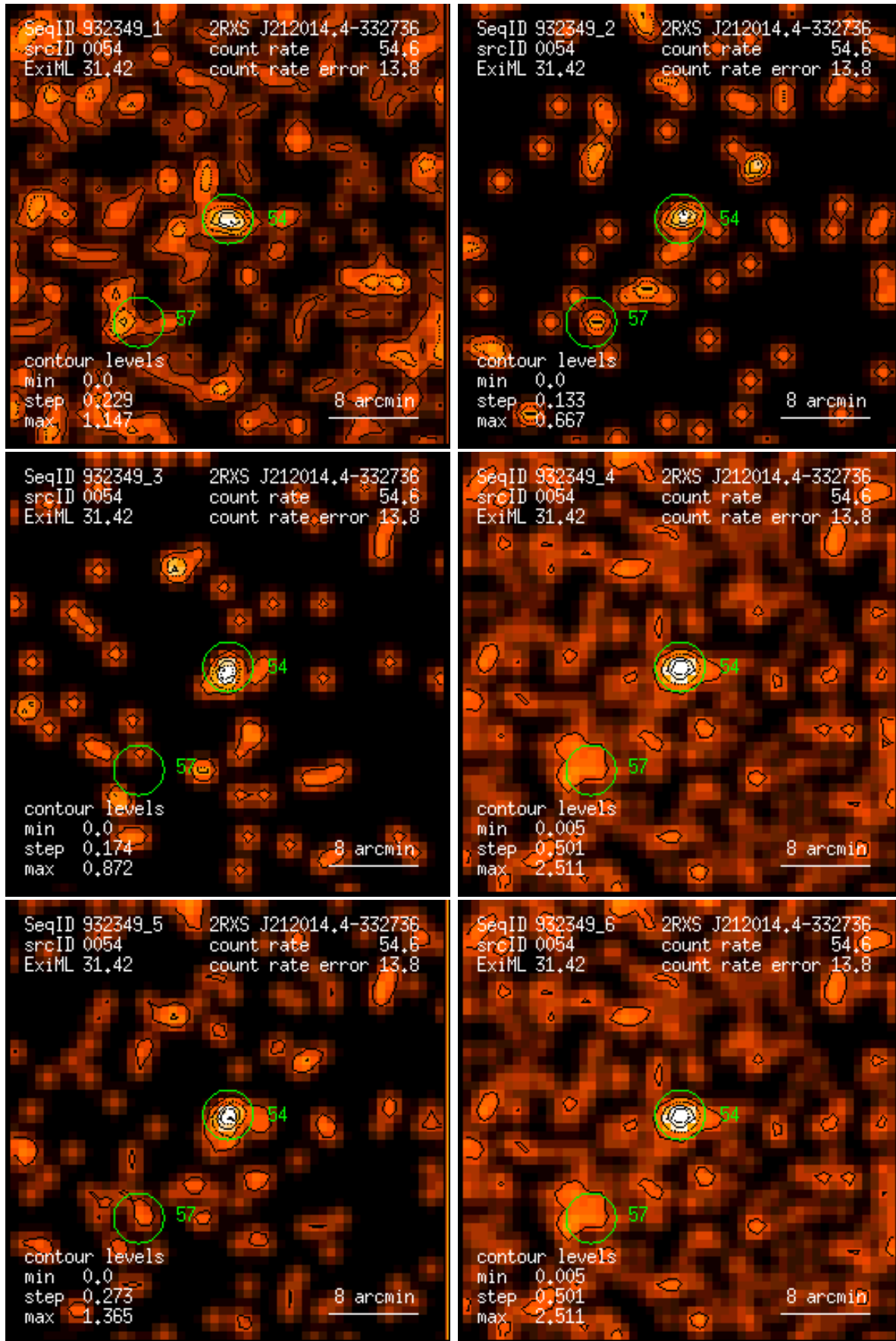
Figure 54: RASS 932349: detection 0054: band rate images, Gaussian filter: (1) PSPC channels 11 – 41, (2) 52 – 90, (3) 91 – 201, (4) 11 – 235, (5) 52 – 201, (6) 11 – 201. Broad band rates in counts/ks. Band rate contour levels in counts/ks/arcmin 2 .
