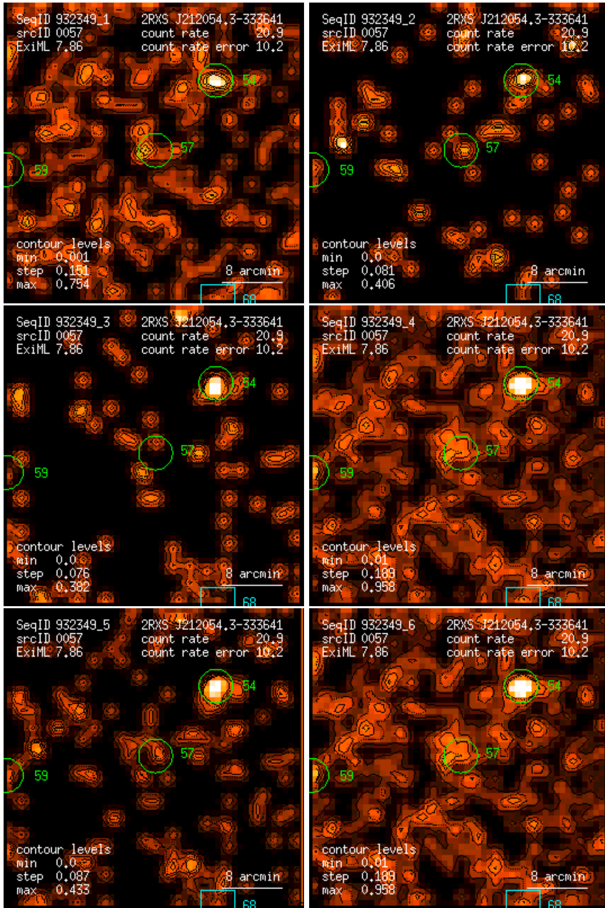
Figure 57: RASS 932349: detection 0057: band rate images, Gaussian filter: (1) PSPC channels 11 – 41, (2) 52 – 90, (3) 91 – 201, (4) 11 – 235, (5) 52 – 201, (6) 11 – 201. Broad band rates in counts/ks. Band rate contour levels in counts/ks/arcmin 2 .
