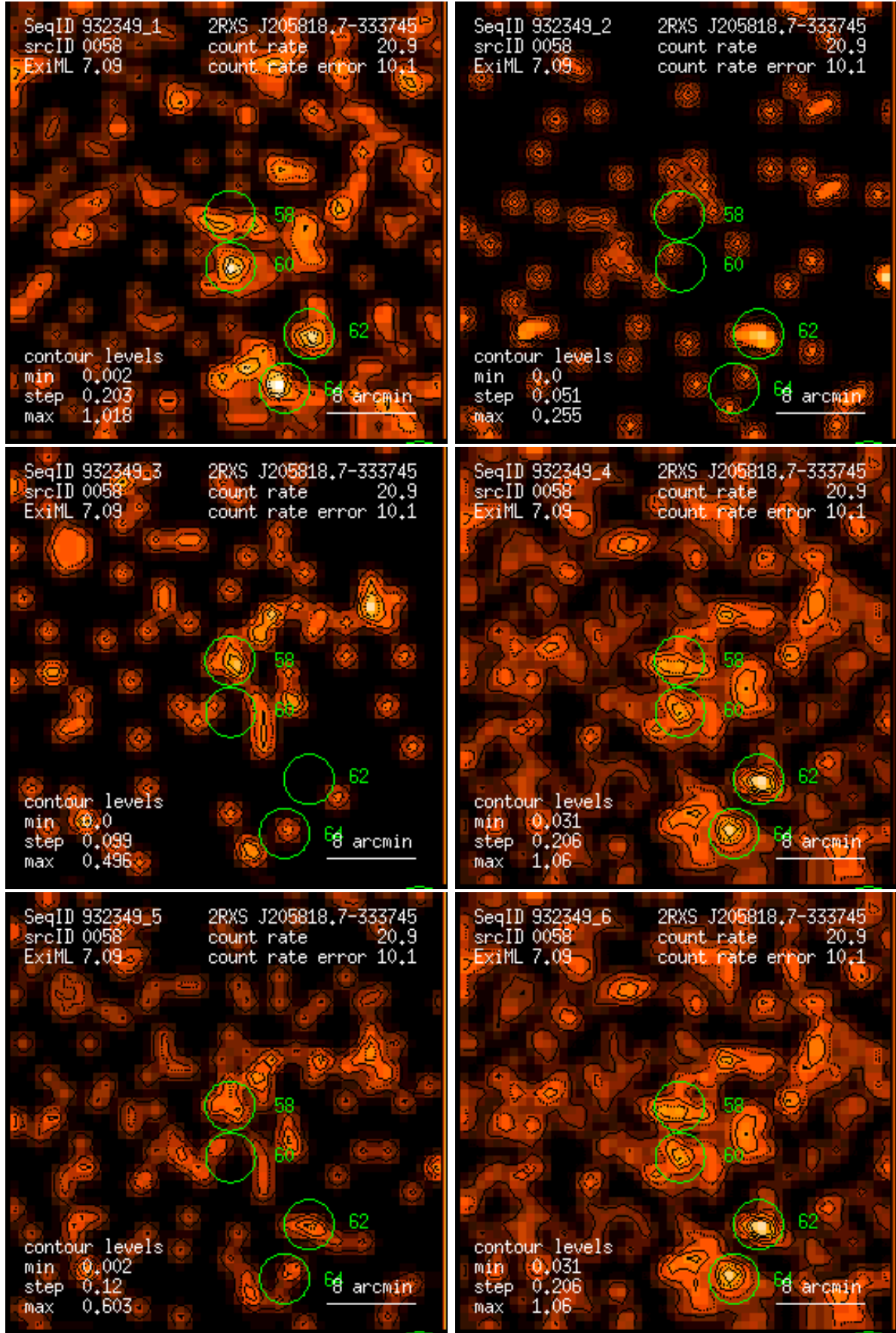
Figure 58: RASS 932349: detection 0058: band rate images, Gaussian filter: (1) PSPC channels 11 – 41, (2) 52 – 90, (3) 91 – 201, (4) 11 – 235, (5) 52 – 201, (6) 11 – 201. Broad band rates in counts/ks. Band rate contour levels in counts/ks/arcmin 2 .
