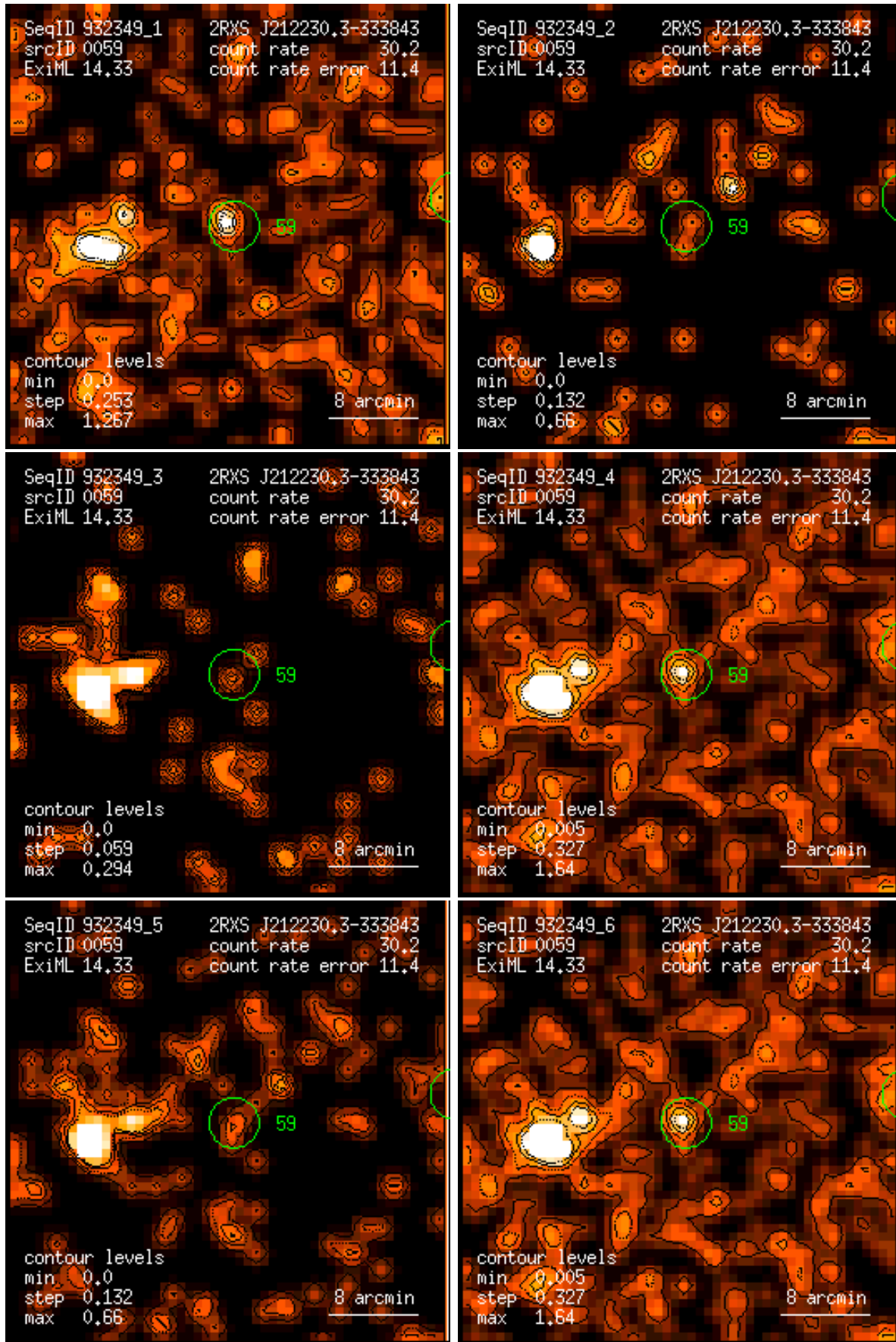
Figure 59: RASS 932349: detection 0059: band rate images, Gaussian filter: (1) PSPC channels 11 – 41, (2) 52 – 90, (3) 91 – 201, (4) 11 – 235, (5) 52 – 201, (6) 11 – 201. Broad band rates in counts/ks. Band rate contour levels in counts/ks/arcmin 2 .
