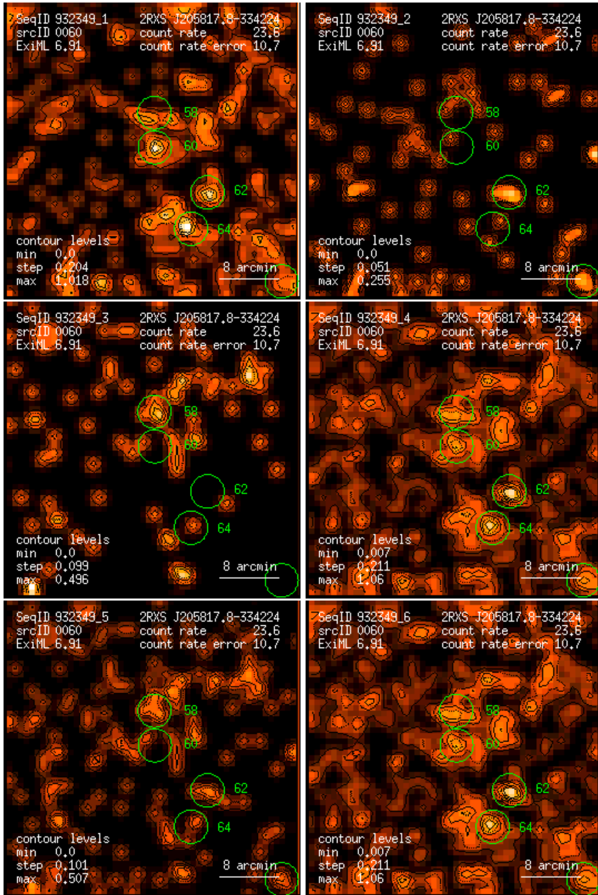
Figure 60: RASS 932349: detection 0060: band rate images, Gaussian filter: (1) PSPC channels 11 – 41, (2) 52 – 90, (3) 91 – 201, (4) 11 – 235, (5) 52 – 201, (6) 11 – 201. Broad band rates in counts/ks. Band rate contour levels in counts/ks/arcmin 2 .
