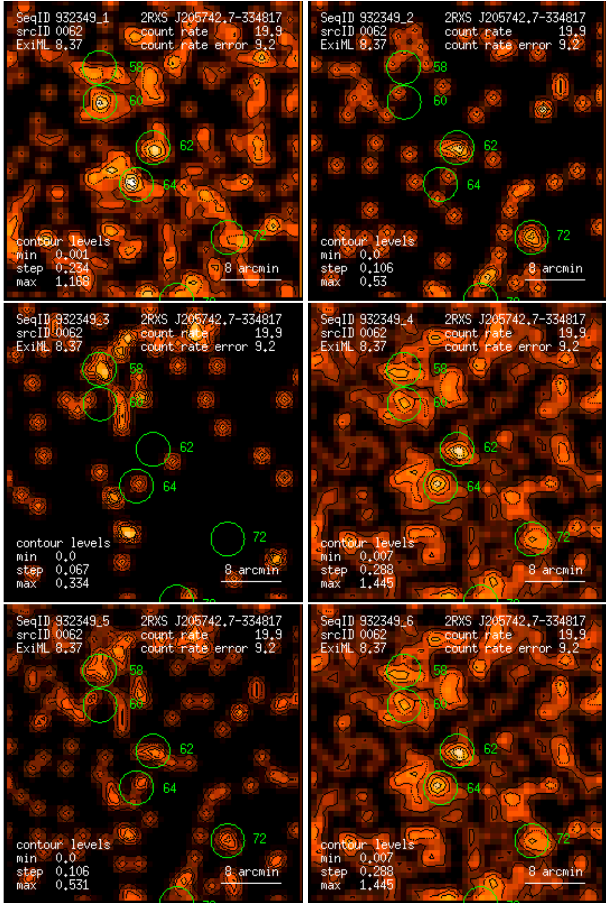
Figure 62: RASS 932349: detection 0062: band rate images, Gaussian filter: (1) PSPC channels 11 – 41, (2) 52 – 90, (3) 91 – 201, (4) 11 – 235, (5) 52 – 201, (6) 11 – 201. Broad band rates in counts/ks. Band rate contour levels in counts/ks/arcmin 2 .
