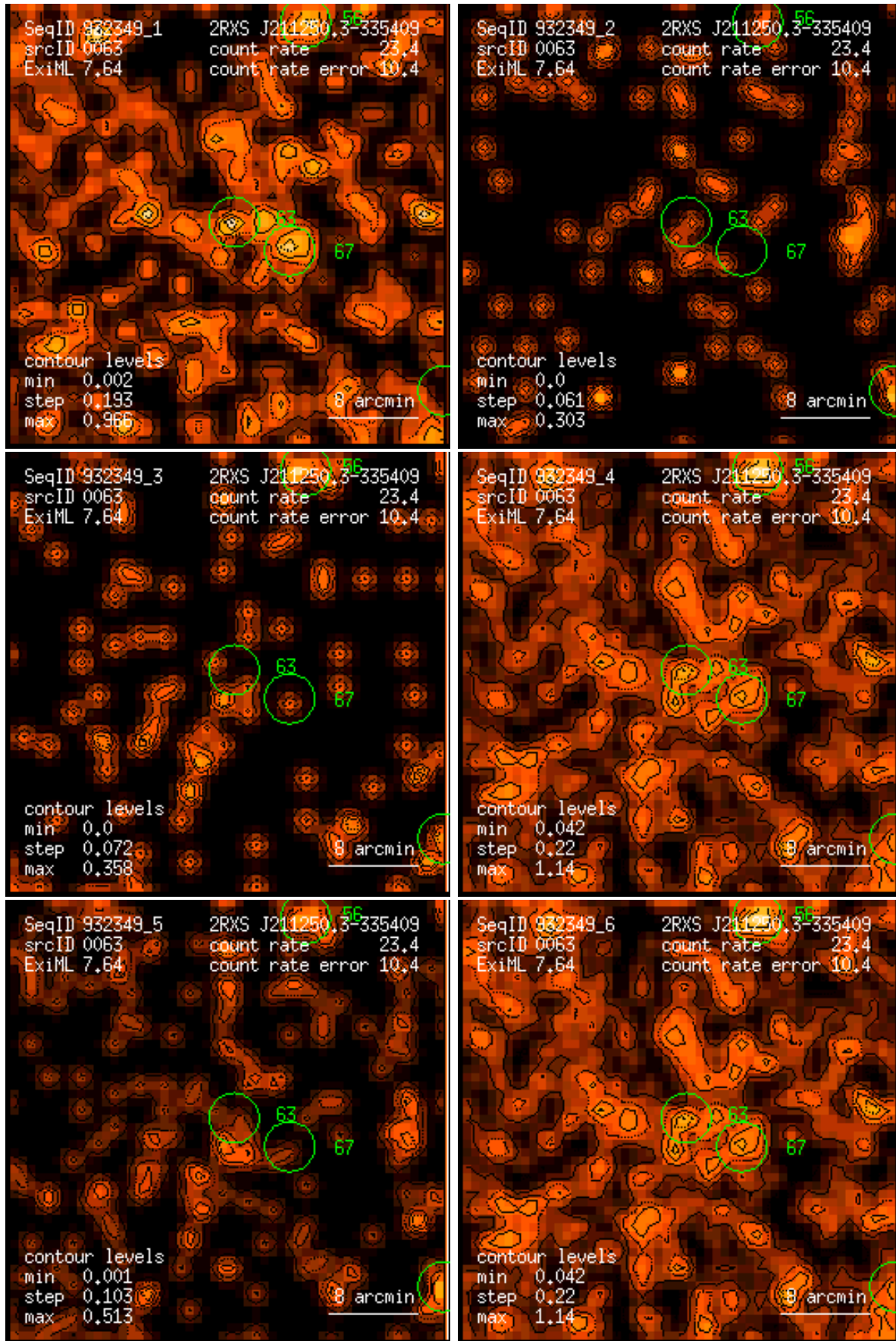
Figure 63: RASS 932349: detection 0063: band rate images, Gaussian filter: (1) PSPC channels 11 – 41, (2) 52 – 90, (3) 91 – 201, (4) 11 – 235, (5) 52 – 201, (6) 11 – 201. Broad band rates in counts/ks. Band rate contour levels in counts/ks/arcmin 2 .
