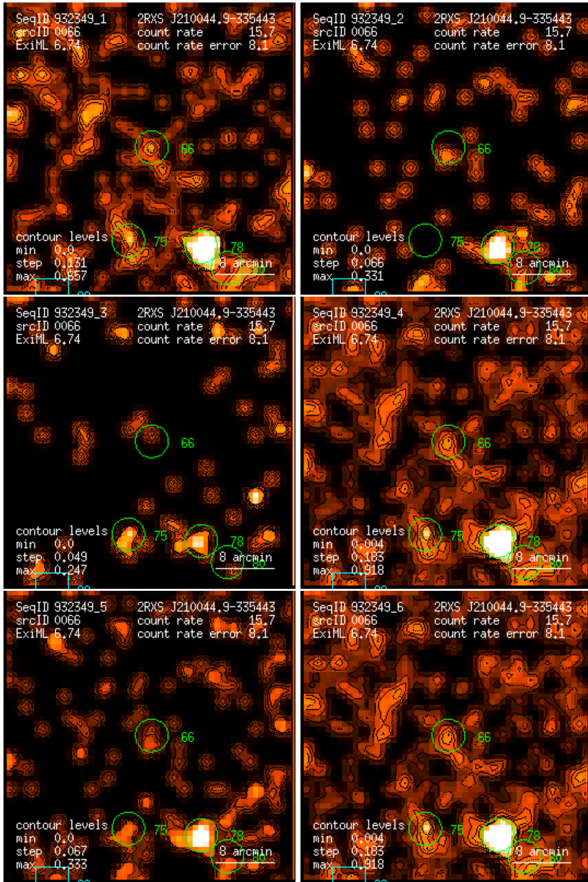
Figure 66: RASS 932349: detection 0066: band rate images, Gaussian filter: (1) PSPC channels 11 – 41, (2) 52 – 90, (3) 91 – 201, (4) 11 – 235, (5) 52 – 201, (6) 11 – 201. Broad band rates in counts/ks. Band rate contour levels in counts/ks/arcmin 2 .
