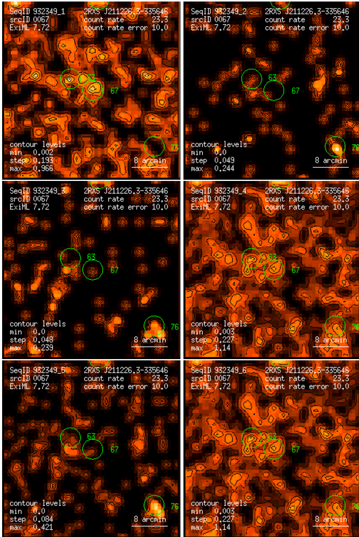
Figure 67: RASS 932349: detection 0067: band rate images, Gaussian filter: (1) PSPC channels 11 – 41, (2) 52 – 90, (3) 91 – 201, (4) 11 – 235, (5) 52 – 201, (6) 11 – 201. Broad band rates in counts/ks. Band rate contour levels in counts/ks/arcmin 2 .
