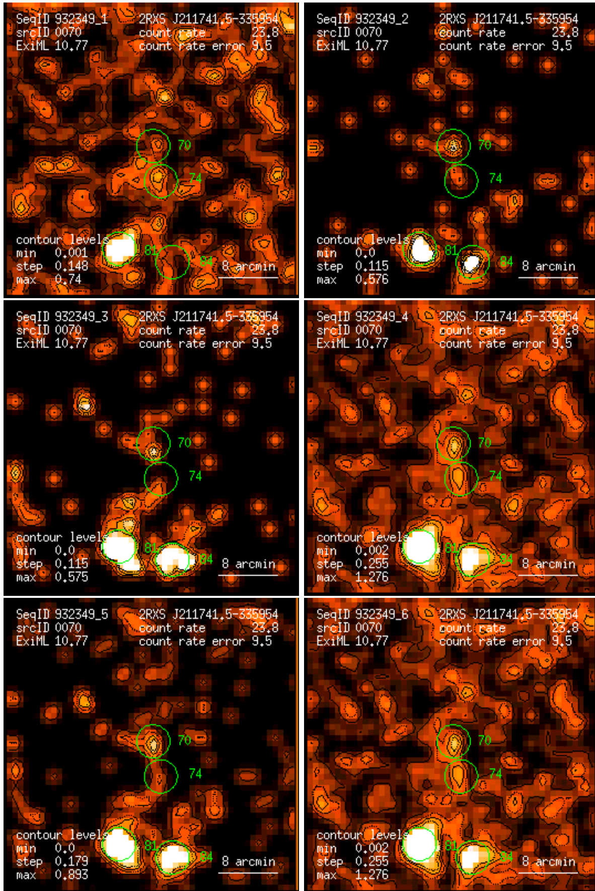
Figure 70: RASS 932349: detection 0070: band rate images, Gaussian filter: (1) PSPC channels 11 – 41, (2) 52 – 90, (3) 91 – 201, (4) 11 – 235, (5) 52 – 201, (6) 11 – 201. Broad band rates in counts/ks. Band rate contour levels in counts/ks/arcmin 2 .
