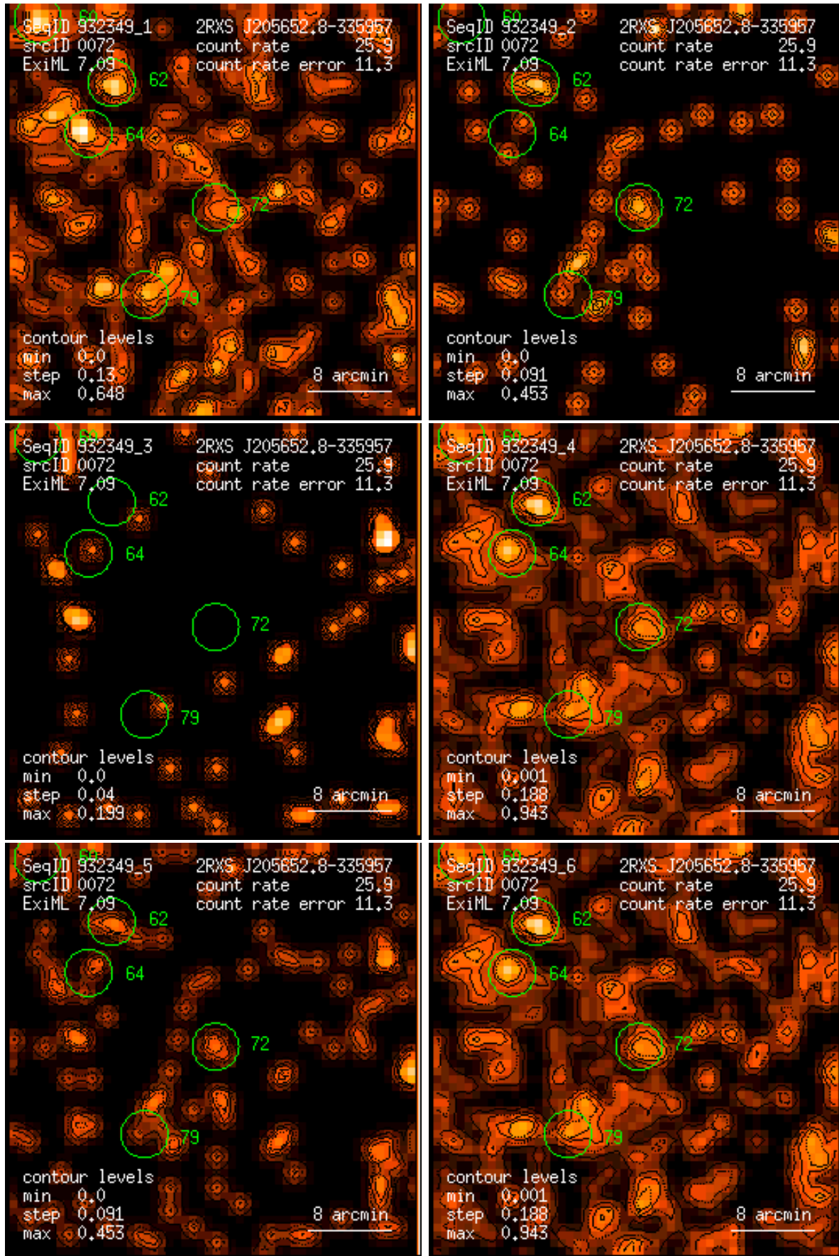
Figure 72: RASS 932349: detection 0072: band rate images, Gaussian filter: (1) PSPC channels 11 – 41, (2) 52 – 90, (3) 91 – 201, (4) 11 – 235, (5) 52 – 201, (6) 11 – 201. Broad band rates in counts/ks. Band rate contour levels in counts/ks/arcmin 2 .
