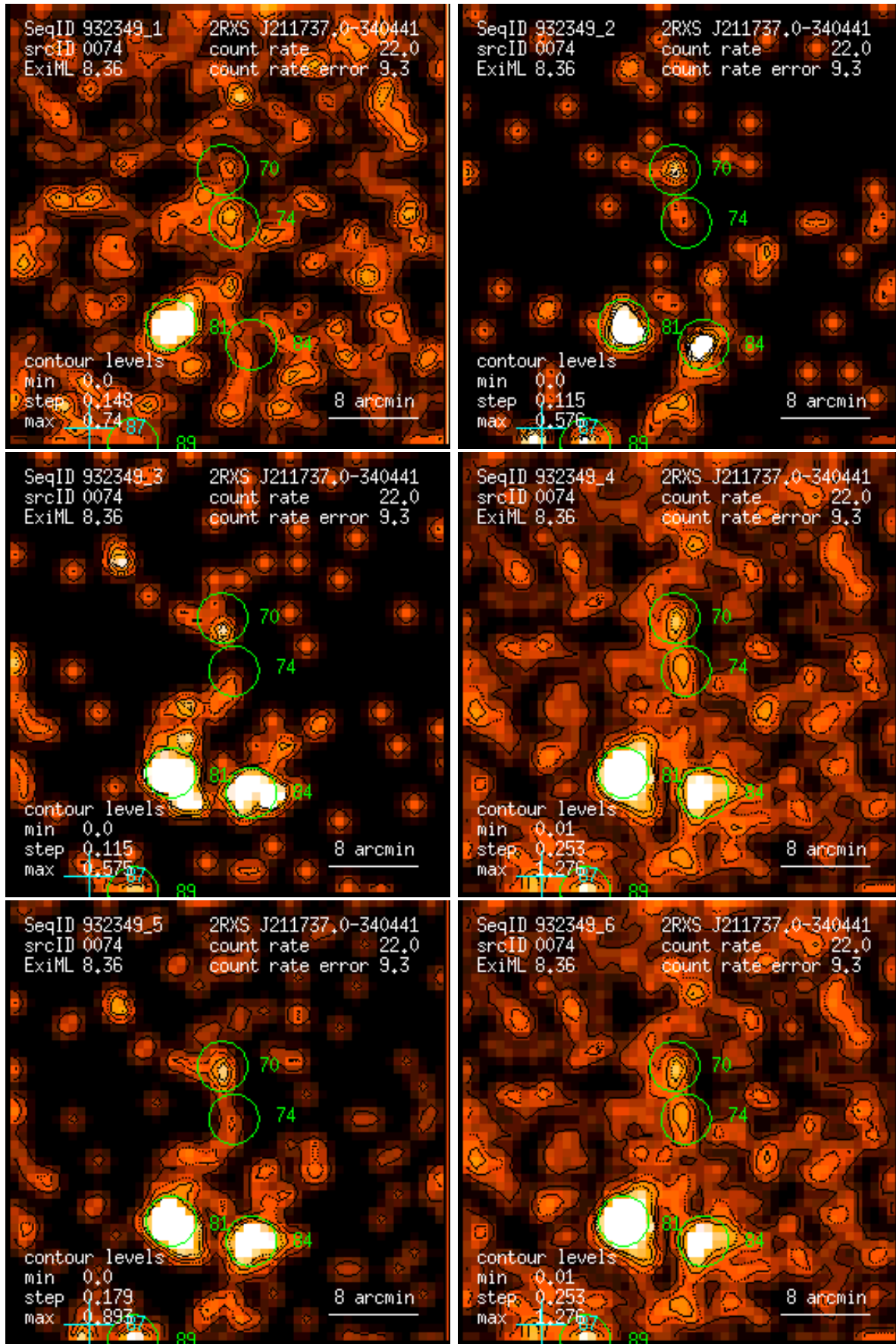
Figure 74: RASS 932349: detection 0074: band rate images, Gaussian filter: (1) PSPC channels 11 – 41, (2) 52 – 90, (3) 91 – 201, (4) 11 – 235, (5) 52 – 201, (6) 11 – 201. Broad band rates in counts/ks. Band rate contour levels in counts/ks/arcmin 2 .
