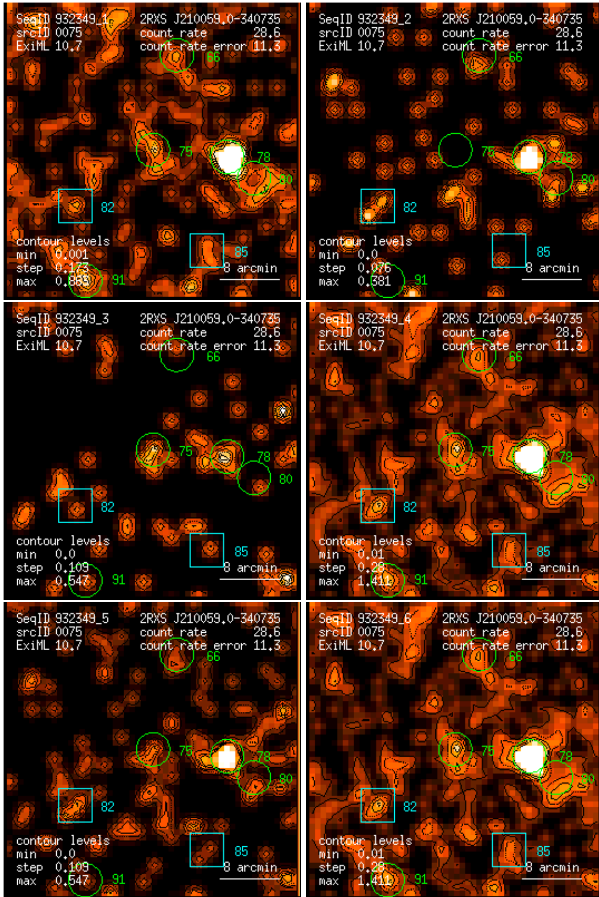
Figure 75: RASS 932349: detection 0075: band rate images, Gaussian filter: (1) PSPC channels 11 – 41, (2) 52 – 90, (3) 91 – 201, (4) 11 – 235, (5) 52 – 201, (6) 11 – 201. Broad band rates in counts/ks. Band rate contour levels in counts/ks/arcmin 2 .
