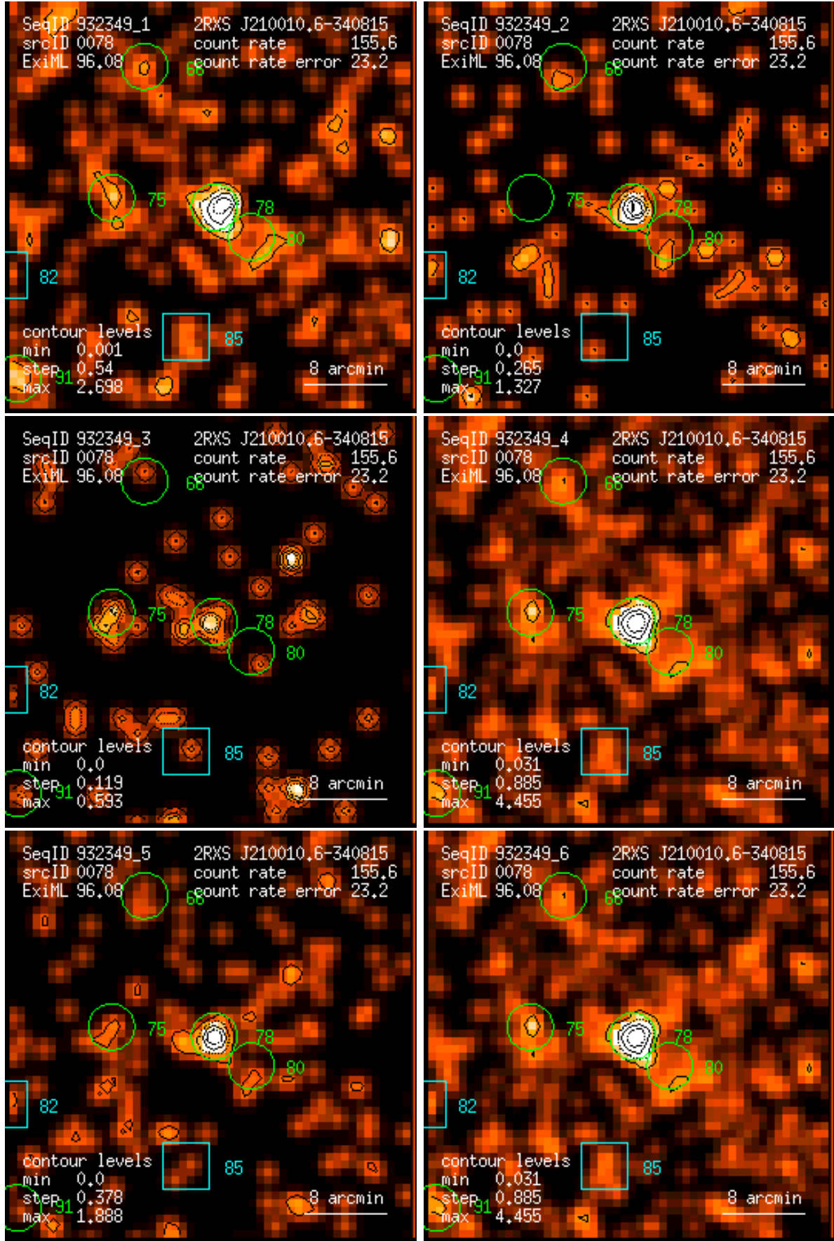
Figure 78: RASS 932349: detection 0078: band rate images, Gaussian filter: (1) PSPC channels 11 – 41, (2) 52 – 90, (3) 91 – 201, (4) 11 – 235, (5) 52 – 201, (6) 11 – 201. Broad band rates in counts/ks. Band rate contour levels in counts/ks/arcmin 2 .
