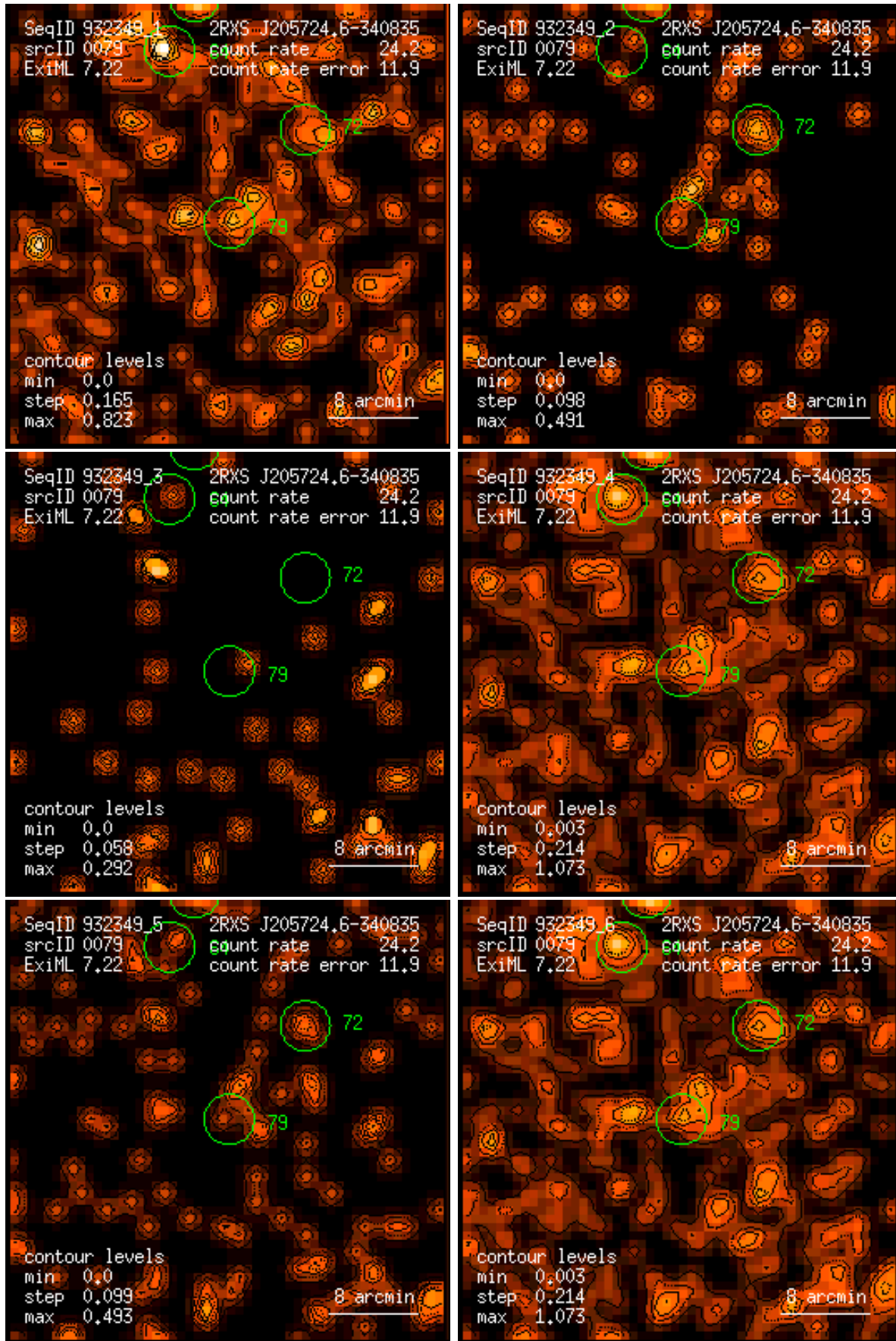
Figure 79: RASS 932349: detection 0079: band rate images, Gaussian filter: (1) PSPC channels 11 – 41, (2) 52 – 90, (3) 91 – 201, (4) 11 – 235, (5) 52 – 201, (6) 11 – 201. Broad band rates in counts/ks. Band rate contour levels in counts/ks/arcmin 2 .
