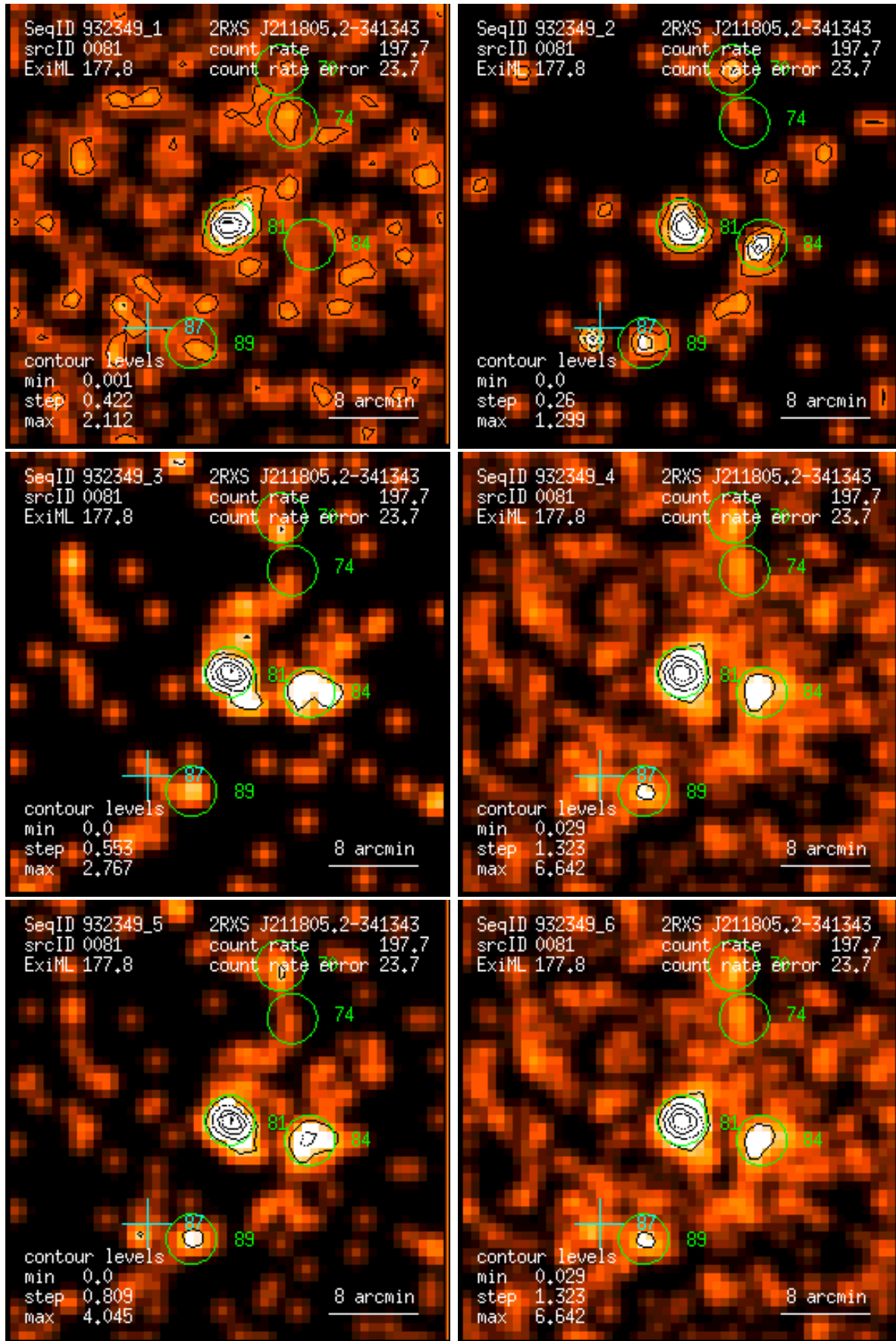
Figure 81: RASS 932349: detection 0081: band rate images, Gaussian filter: (1) PSPC channels 11 – 41, (2) 52 – 90, (3) 91 – 201, (4) 11 – 235, (5) 52 – 201, (6) 11 – 201. Broad band rates in counts/ks. Band rate contour levels in counts/ks/arcmin 2 .
