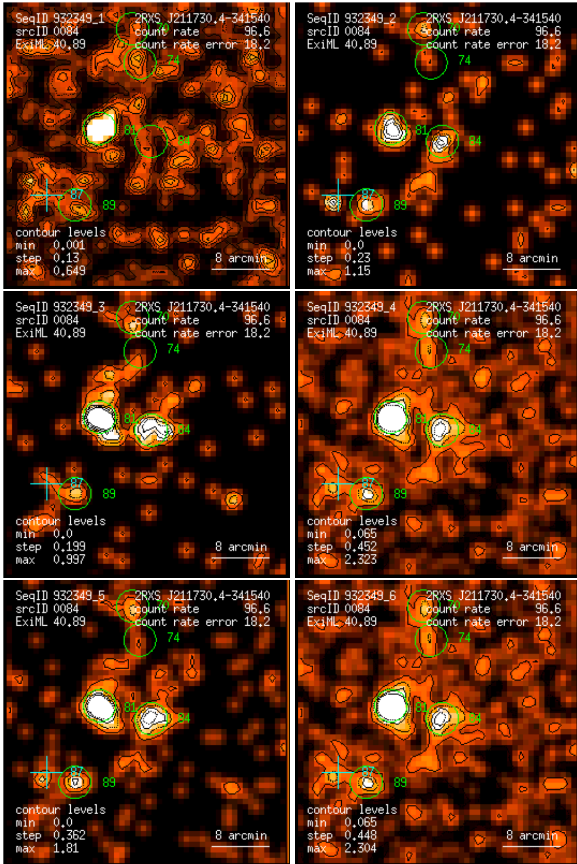
Figure 84: RASS 932349: detection 0084: band rate images, Gaussian filter: (1) PSPC channels 11 – 41, (2) 52 – 90, (3) 91 – 201, (4) 11 – 235, (5) 52 – 201, (6) 11 – 201. Broad band rates in counts/ks. Band rate contour levels in counts/ks/arcmin 2 .
