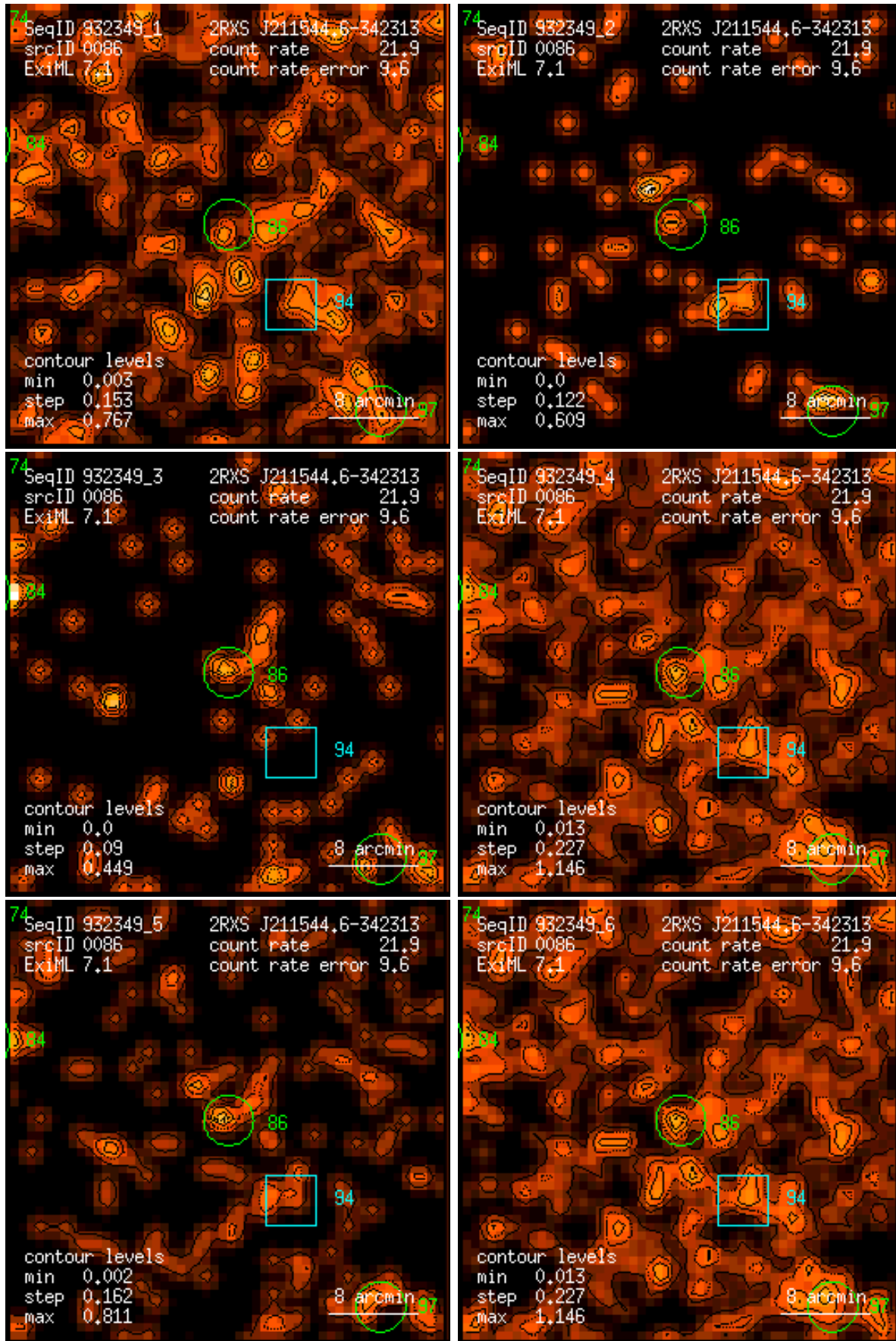
Figure 86: RASS 932349: detection 0086: band rate images, Gaussian filter: (1) PSPC channels 11 – 41, (2) 52 – 90, (3) 91 – 201, (4) 11 – 235, (5) 52 – 201, (6) 11 – 201. Broad band rates in counts/ks. Band rate contour levels in counts/ks/arcmin 2 .
