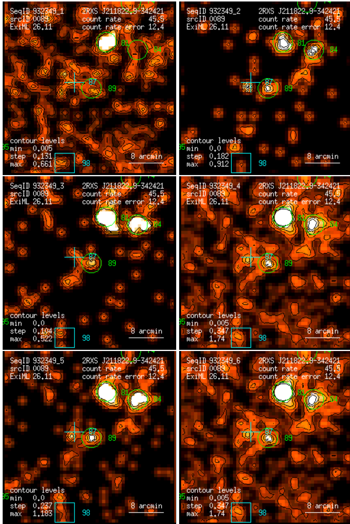
Figure 89: RASS 932349: detection 0089: band rate images, Gaussian filter: (1) PSPC channels 11 – 41, (2) 52 – 90, (3) 91 – 201, (4) 11 – 235, (5) 52 – 201, (6) 11 – 201. Broad band rates in counts/ks. Band rate contour levels in counts/ks/arcmin 2 .
