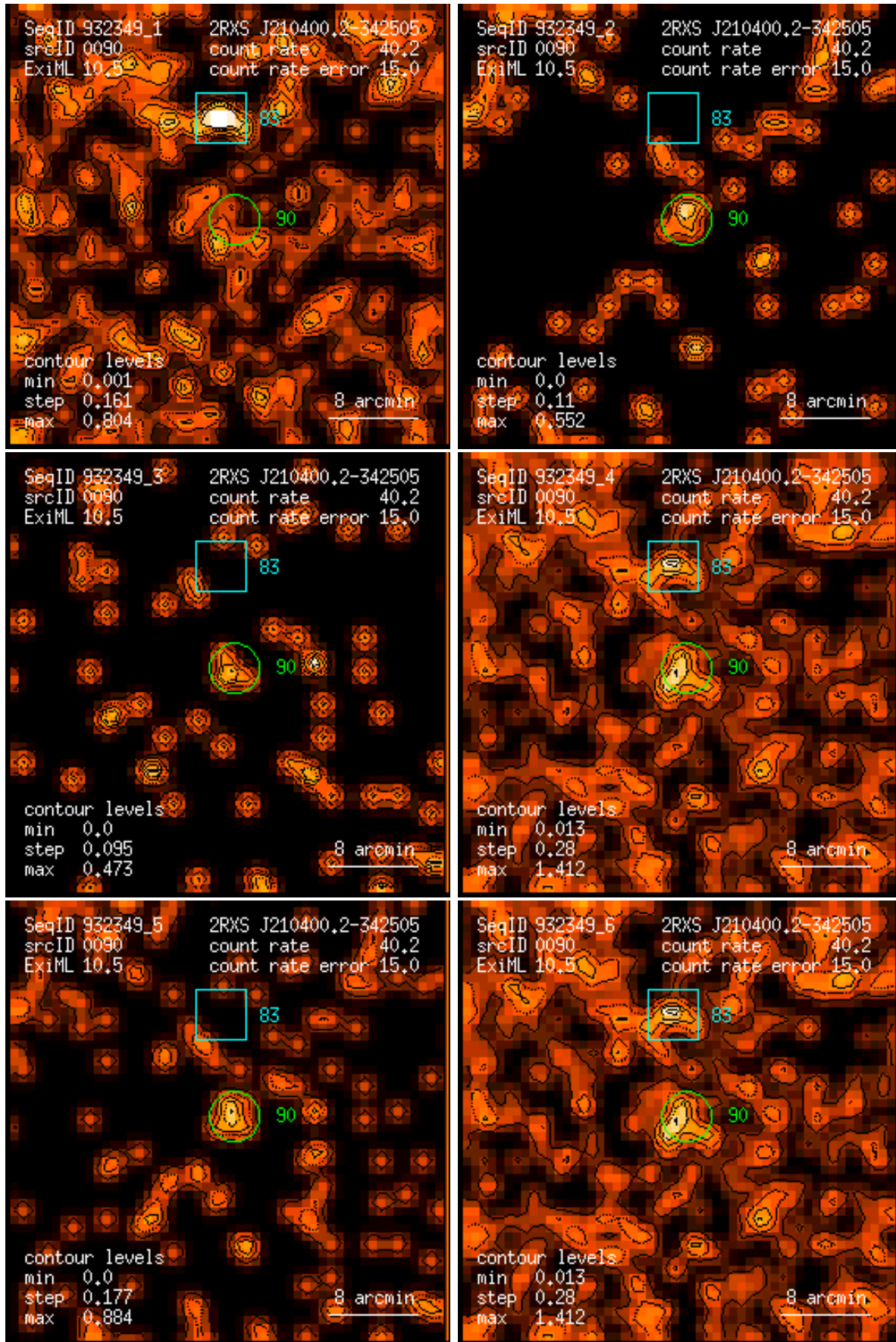
Figure 90: RASS 932349: detection 0090: band rate images, Gaussian filter: (1) PSPC channels 11 – 41, (2) 52 – 90, (3) 91 – 201, (4) 11 – 235, (5) 52 – 201, (6) 11 – 201. Broad band rates in counts/ks. Band rate contour levels in counts/ks/arcmin 2 .
