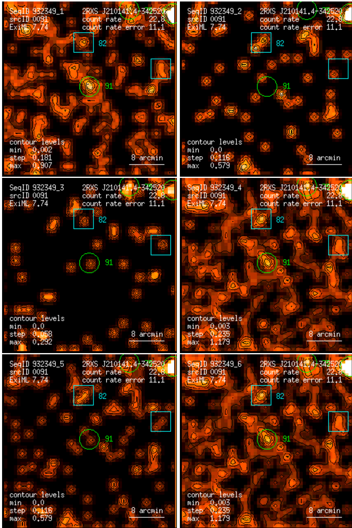
Figure 91: RASS 932349: detection 0091: band rate images, Gaussian filter: (1) PSPC channels 11 – 41, (2) 52 – 90, (3) 91 – 201, (4) 11 – 235, (5) 52 – 201, (6) 11 – 201. Broad band rates in counts/ks. Band rate contour levels in counts/ks/arcmin 2 .
