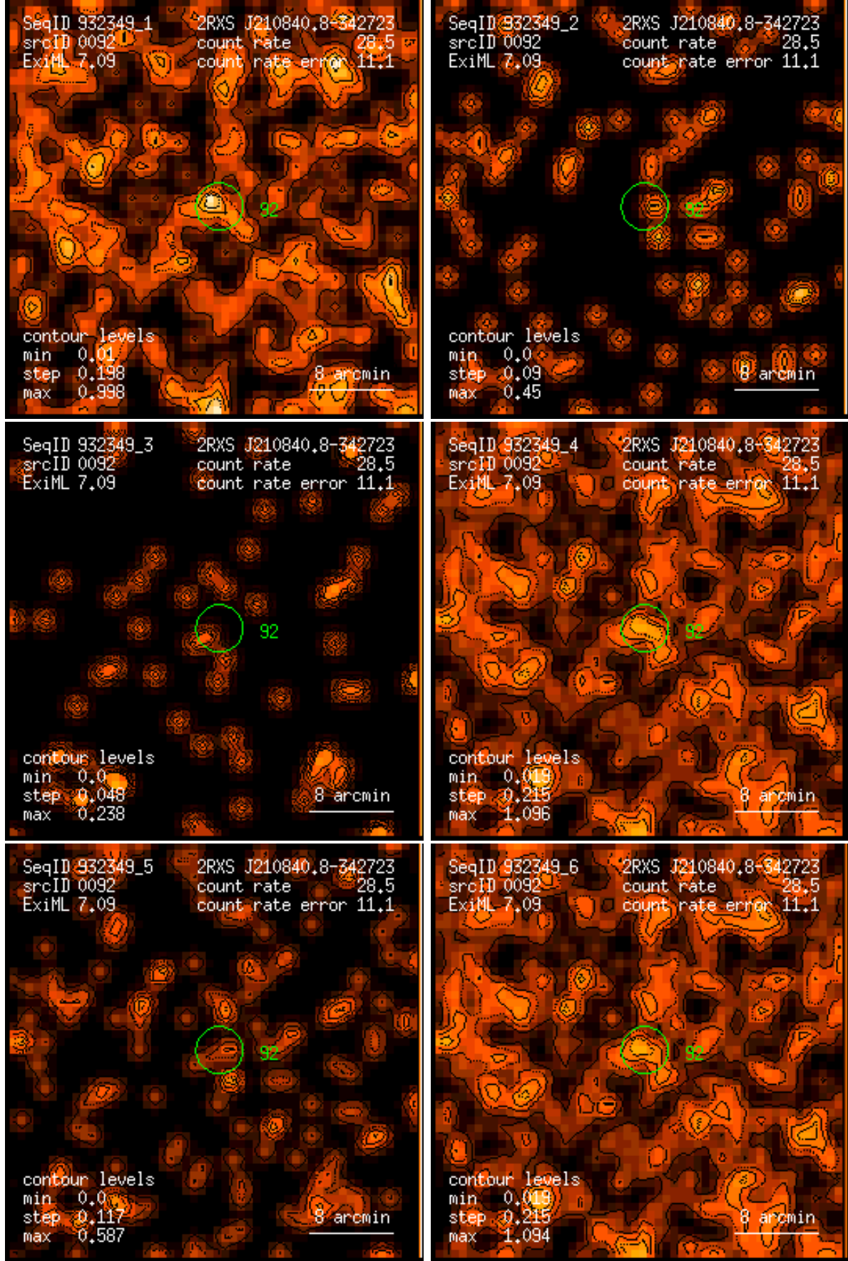
Figure 92: RASS 932349: detection 0092: band rate images, Gaussian filter: (1) PSPC channels 11 – 41, (2) 52 – 90, (3) 91 – 201, (4) 11 – 235, (5) 52 – 201, (6) 11 – 201. Broad band rates in counts/ks. Band rate contour levels in counts/ks/arcmin 2 .
