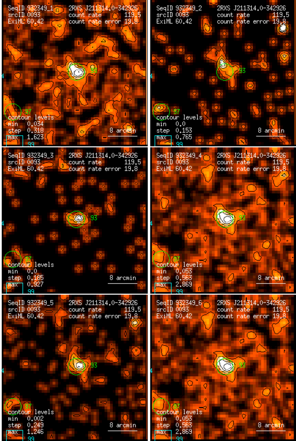
Figure 93: RASS 932349: detection 0093: band rate images, Gaussian filter: (1) PSPC channels 11 – 41, (2) 52 – 90, (3) 91 – 201, (4) 11 – 235, (5) 52 – 201, (6) 11 – 201. Broad band rates in counts/ks. Band rate contour levels in counts/ks/arcmin 2 .
