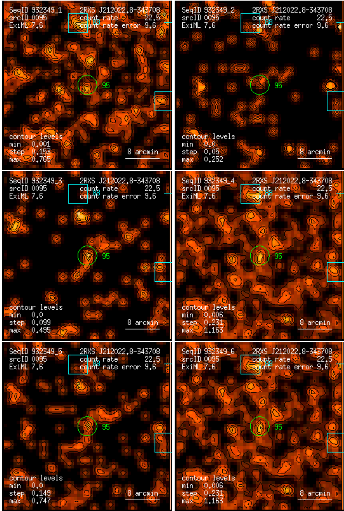
Figure 95: RASS 932349: detection 0095: band rate images, Gaussian filter: (1) PSPC channels 11 – 41, (2) 52 – 90, (3) 91 – 201, (4) 11 – 235, (5) 52 – 201, (6) 11 – 201. Broad band rates in counts/ks. Band rate contour levels in counts/ks/arcmin 2 .
