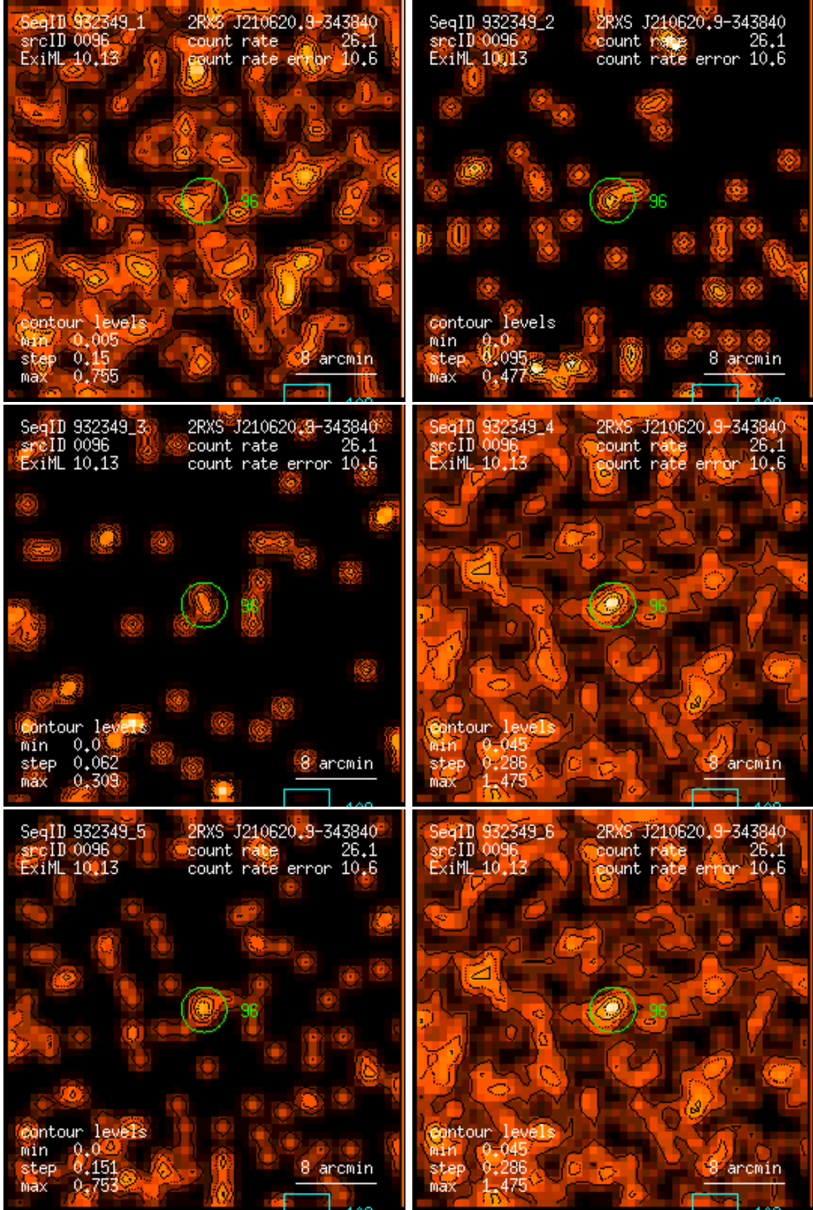
Figure 96: RASS 932349: detection 0096: band rate images, Gaussian filter: (1) PSPC channels 11 – 41, (2) 52 – 90, (3) 91 – 201, (4) 11 – 235, (5) 52 – 201, (6) 11 – 201. Broad band rates in counts/ks. Band rate contour levels in counts/ks/arcmin 2 .
