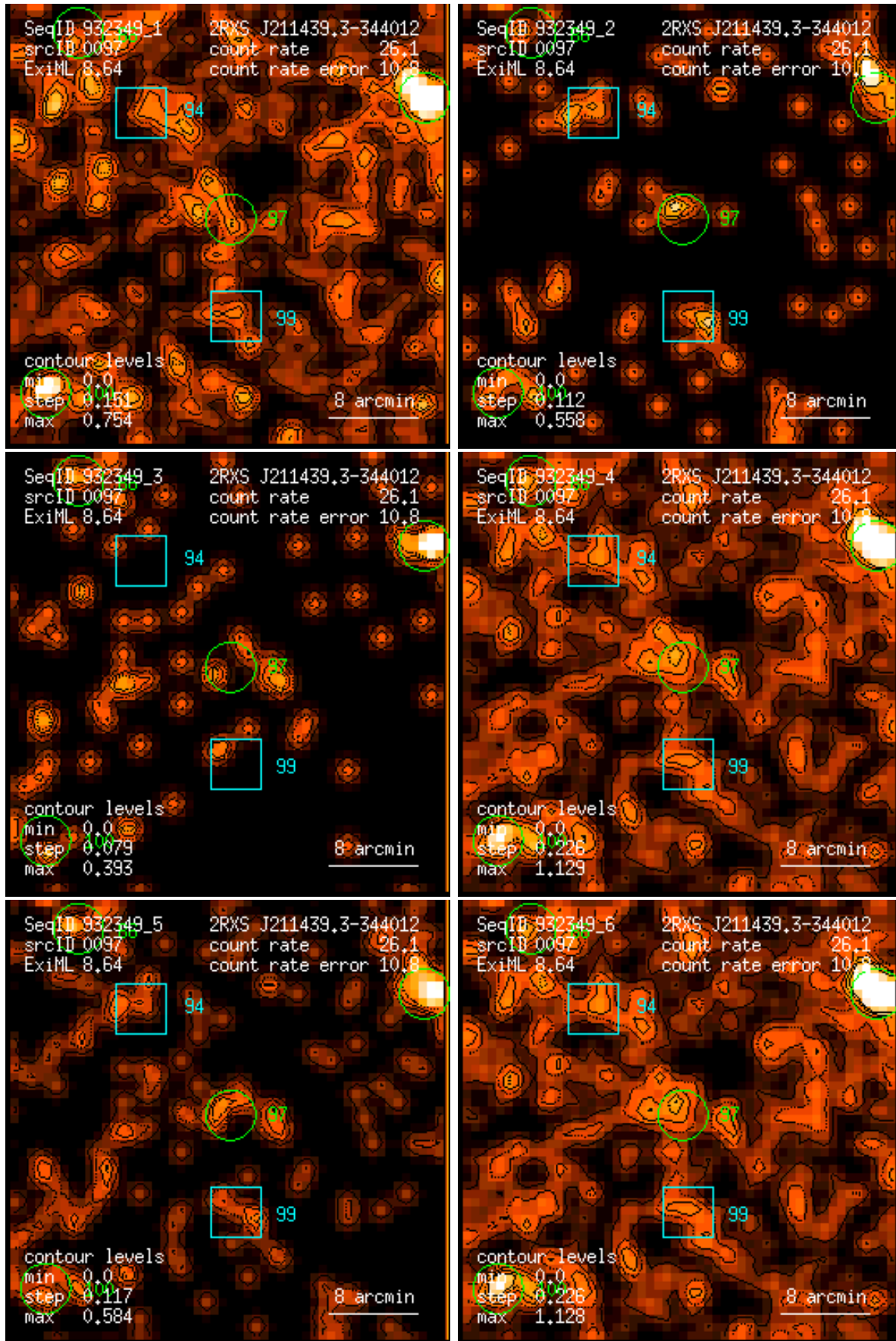
Figure 97: RASS 932349: detection 0097: band rate images, Gaussian filter: (1) PSPC channels 11 – 41, (2) 52 – 90, (3) 91 – 201, (4) 11 – 235, (5) 52 – 201, (6) 11 – 201. Broad band rates in counts/ks. Band rate contour levels in counts/ks/arcmin 2 .
