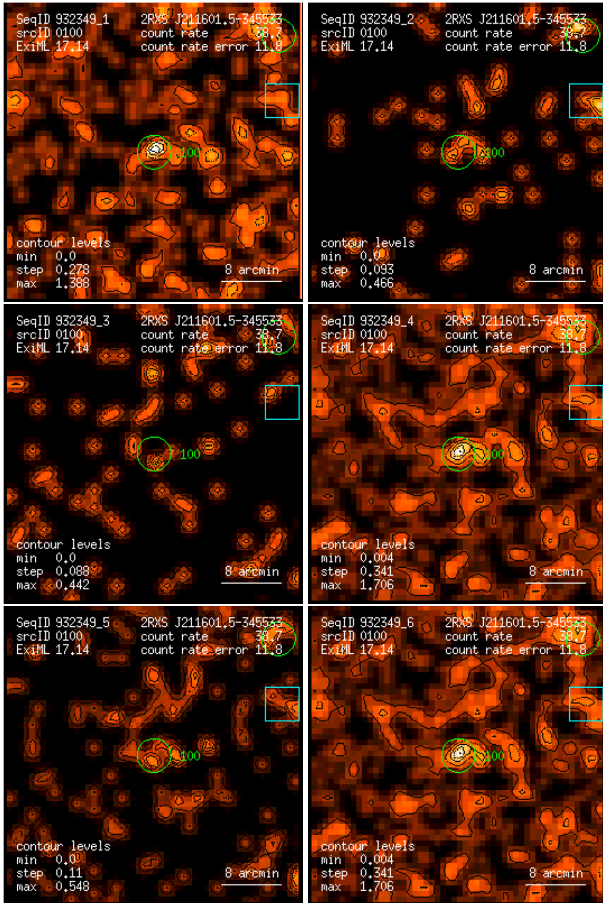
Figure 100: RASS 932349: detection 0100: band rate images, Gaussian filter: (1) PSPC channels 11 – 41, (2) 52 – 90, (3) 91 – 201, (4) 11 – 235, (5) 52 – 201, (6) 11 – 201. Broad band rates in counts/ks. Band rate contour levels in counts/ks/arcmin 2 .
