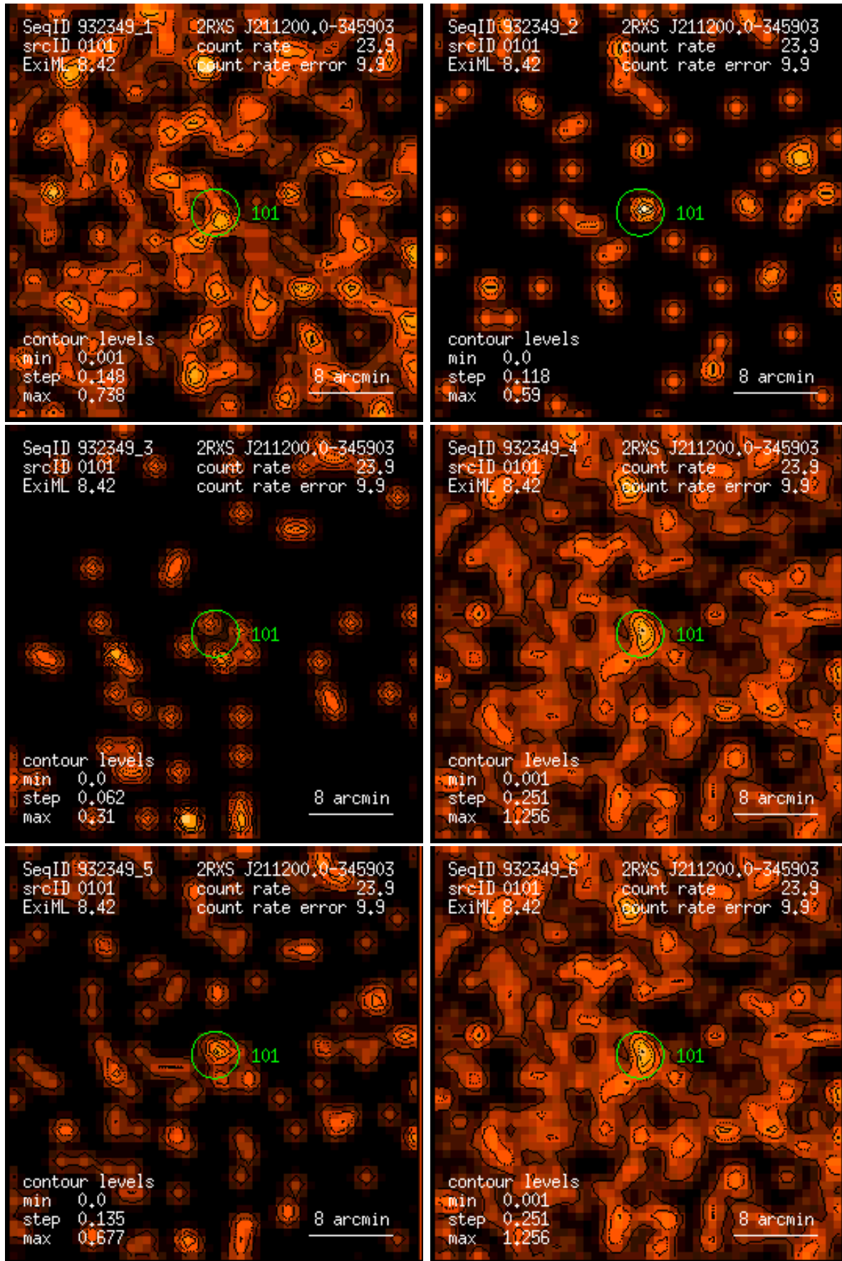
Figure 101: RASS 932349: detection 0101: band rate images, Gaussian filter: (1) PSPC channels 11 – 41, (2) 52 – 90, (3) 91 – 201, (4) 11 – 235, (5) 52 – 201, (6) 11 – 201. Broad band rates in counts/ks. Band rate contour levels in counts/ks/arcmin 2 .
