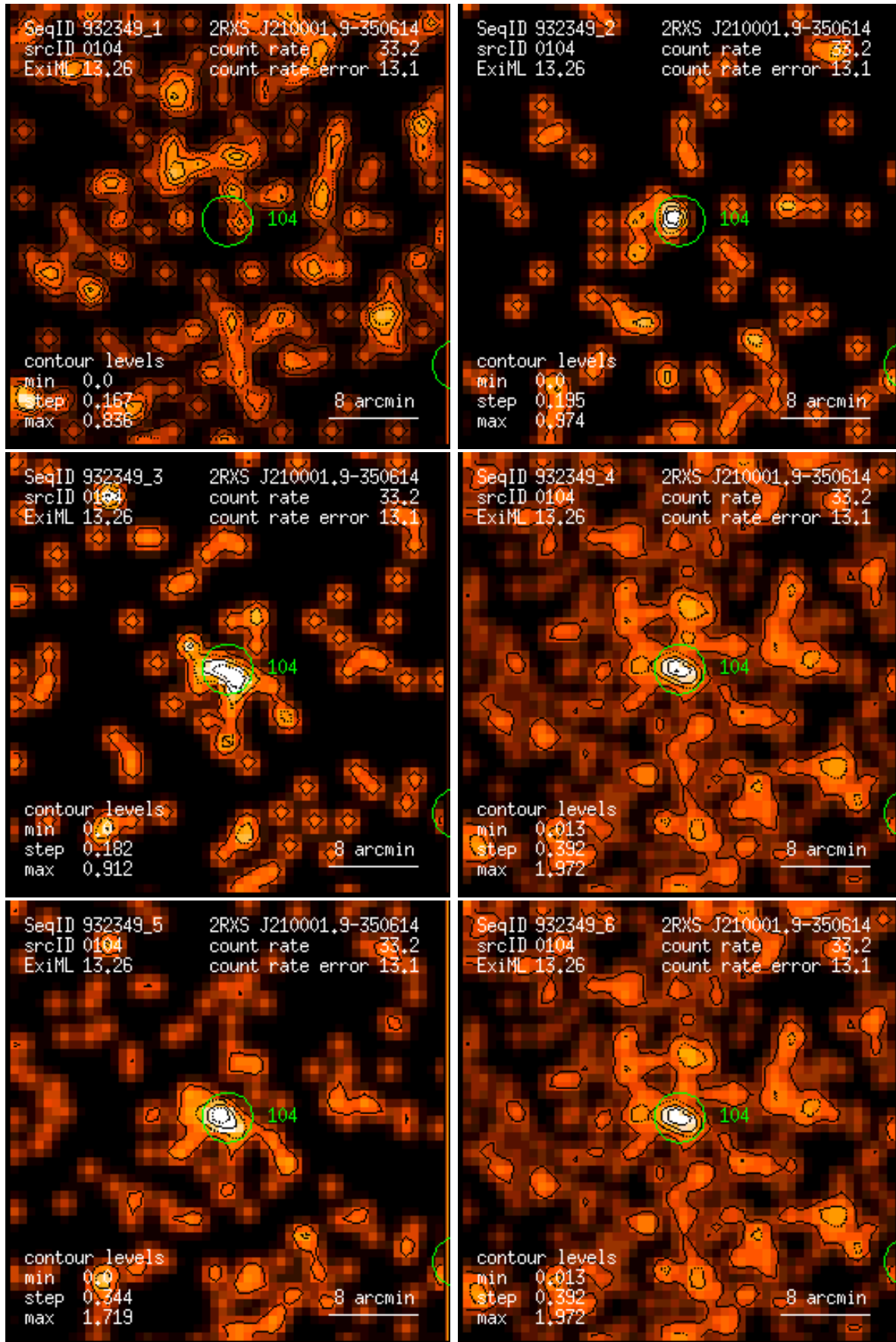
Figure 104: RASS 932349: detection 0104: band rate images, Gaussian filter: (1) PSPC channels 11 – 41, (2) 52 – 90, (3) 91 – 201, (4) 11 – 235, (5) 52 – 201, (6) 11 – 201. Broad band rates in counts/ks. Band rate contour levels in counts/ks/arcmin 2 .
