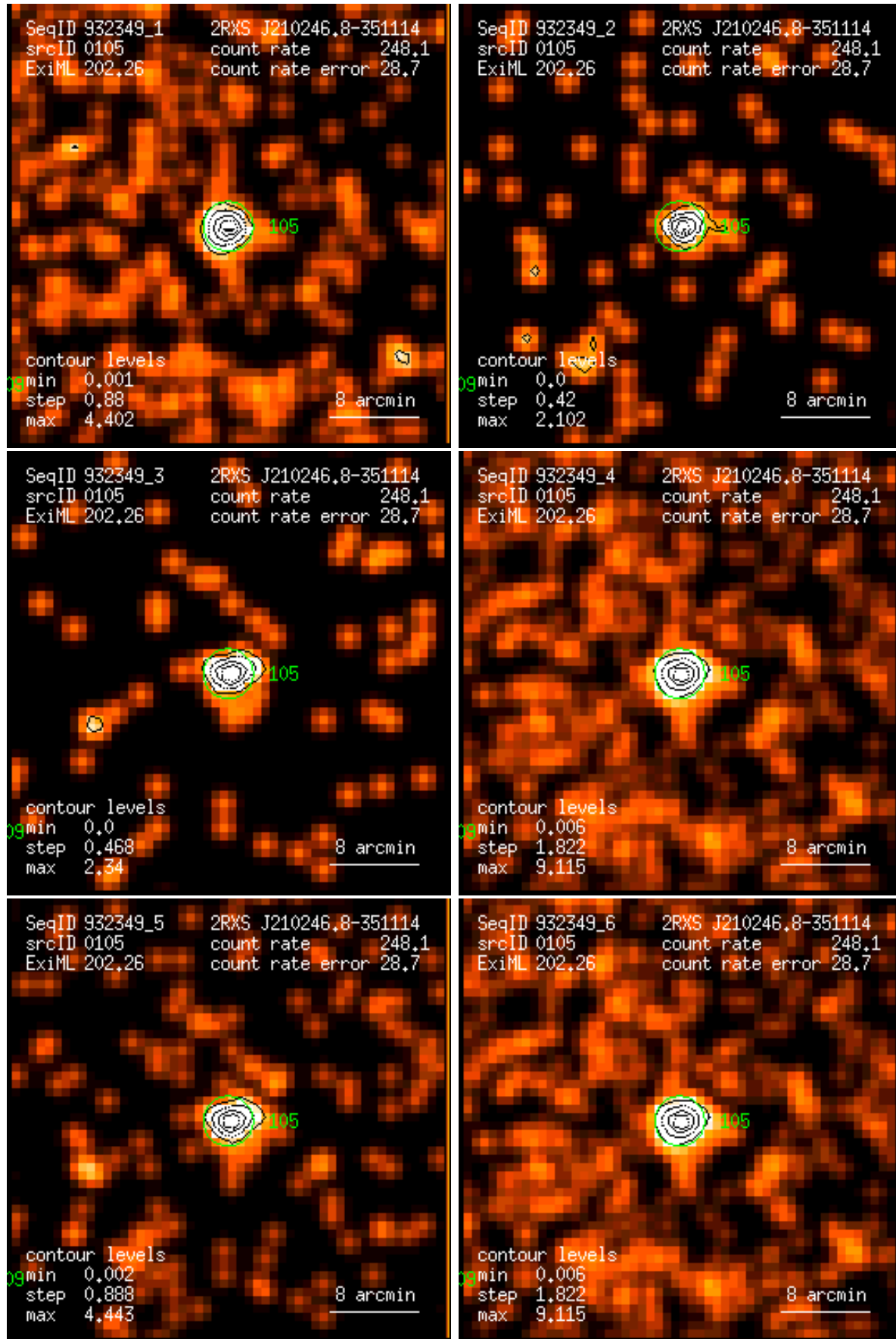
Figure 105: RASS 932349: detection 0105: band rate images, Gaussian filter: (1) PSPC channels 11 – 41, (2) 52 – 90, (3) 91 – 201, (4) 11 – 235, (5) 52 – 201, (6) 11 – 201. Broad band rates in counts/ks. Band rate contour levels in counts/ks/arcmin 2 .
