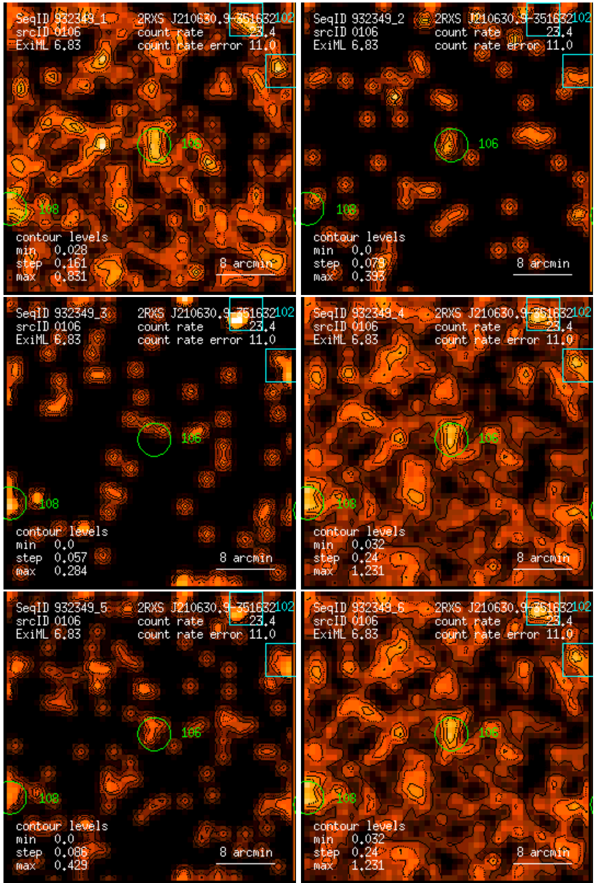
Figure 106: RASS 932349: detection 0106: band rate images, Gaussian filter: (1) PSPC channels 11 – 41, (2) 52 – 90, (3) 91 – 201, (4) 11 – 235, (5) 52 – 201, (6) 11 – 201. Broad band rates in counts/ks. Band rate contour levels in counts/ks/arcmin 2 .
