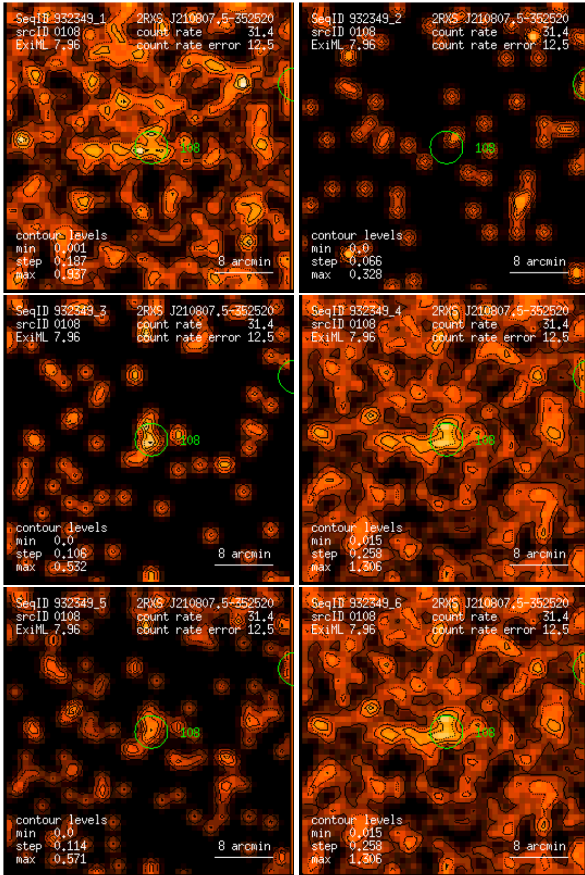
Figure 108: RASS 932349: detection 0108: band rate images, Gaussian filter: (1) PSPC channels 11 – 41, (2) 52 – 90, (3) 91 – 201, (4) 11 – 235, (5) 52 – 201, (6) 11 – 201. Broad band rates in counts/ks. Band rate contour levels in counts/ks/arcmin 2 .
