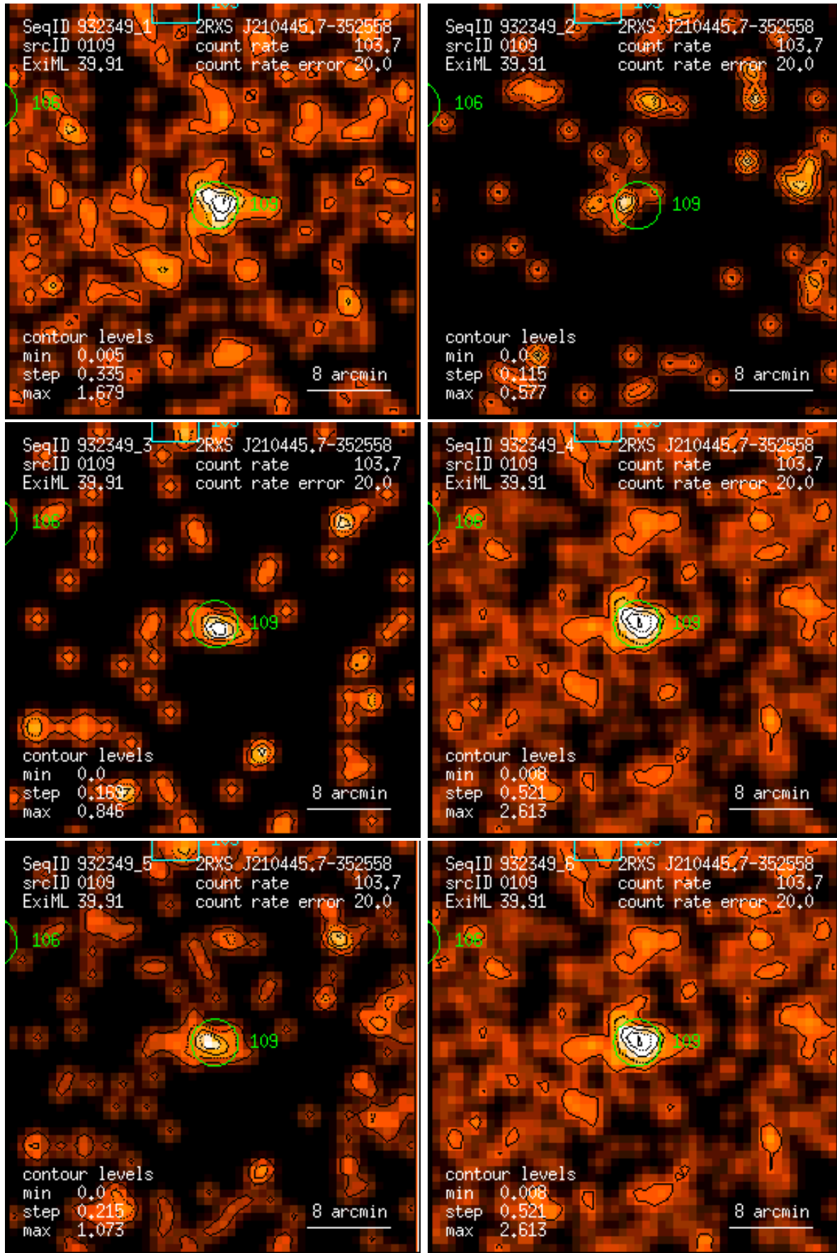
Figure 109: RASS 932349: detection 0109: band rate images, Gaussian filter: (1) PSPC channels 11 – 41, (2) 52 – 90, (3) 91 – 201, (4) 11 – 235, (5) 52 – 201, (6) 11 – 201. Broad band rates in counts/ks. Band rate contour levels in counts/ks/arcmin 2 .
