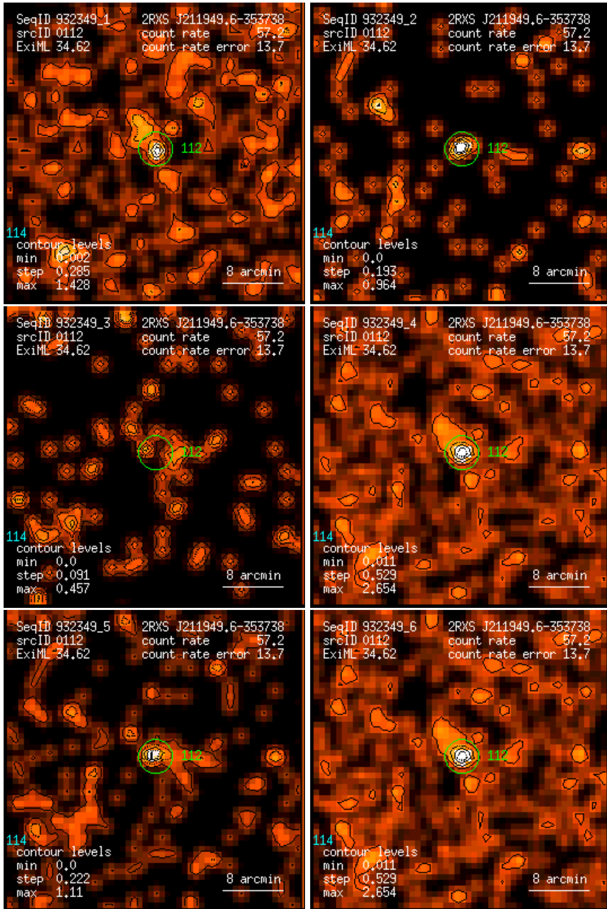
Figure 112: RASS 932349: detection 0112: band rate images, Gaussian filter: (1) PSPC channels 11 – 41, (2) 52 – 90, (3) 91 – 201, (4) 11 – 235, (5) 52 – 201, (6) 11 – 201. Broad band rates in counts/ks. Band rate contour levels in counts/ks/arcmin 2 .
