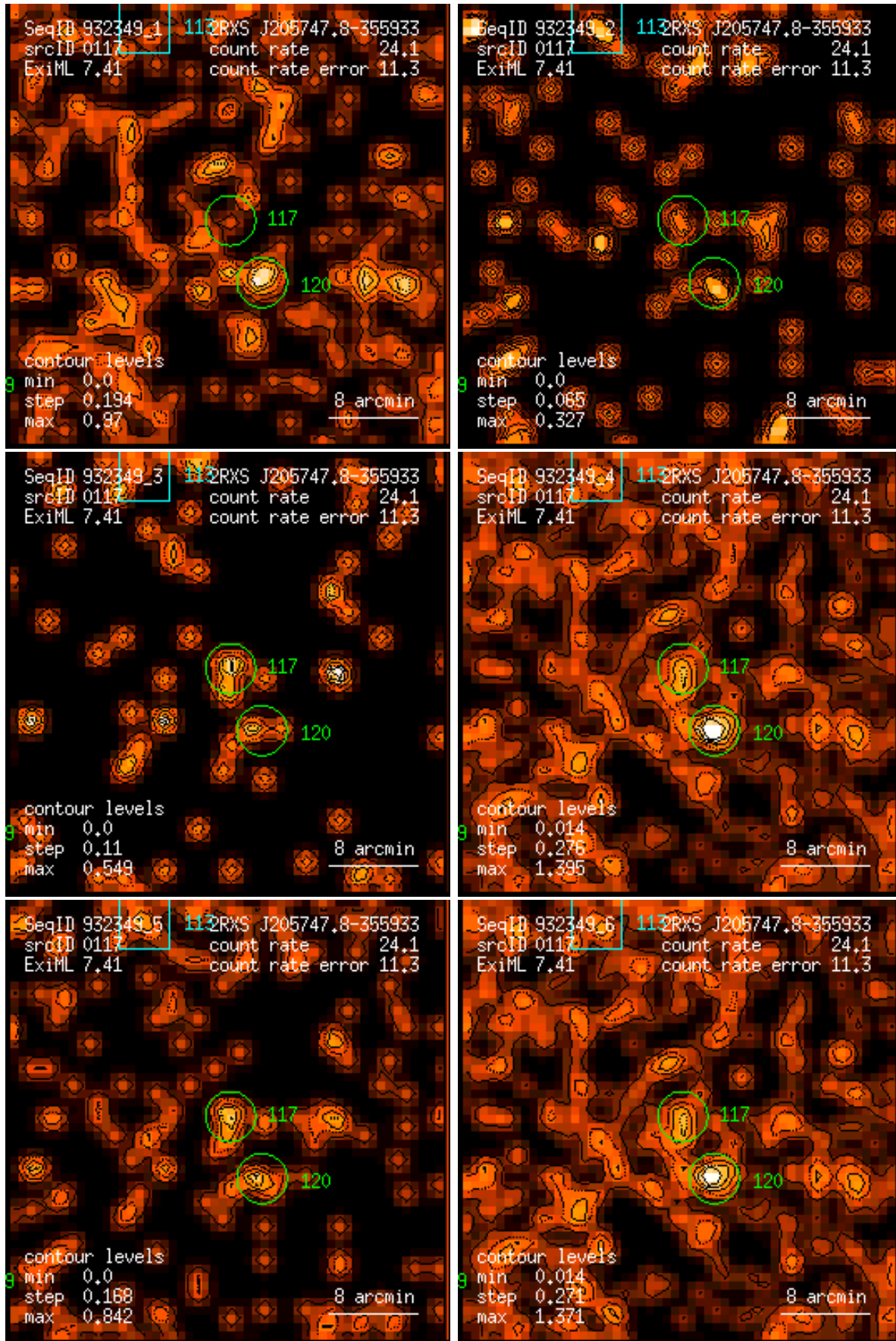
Figure 117: RASS 932349: detection 0117: band rate images, Gaussian filter: (1) PSPC channels 11 – 41, (2) 52 – 90, (3) 91 – 201, (4) 11 – 235, (5) 52 – 201, (6) 11 – 201. Broad band rates in counts/ks. Band rate contour levels in counts/ks/arcmin 2 .
