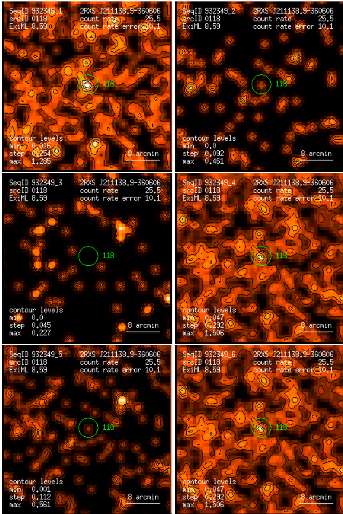
Figure 118: RASS 932349: detection 0118: band rate images, Gaussian filter: (1) PSPC channels 11 – 41, (2) 52 – 90, (3) 91 – 201, (4) 11 – 235, (5) 52 – 201, (6) 11 – 201. Broad band rates in counts/ks. Band rate contour levels in counts/ks/arcmin 2 .
