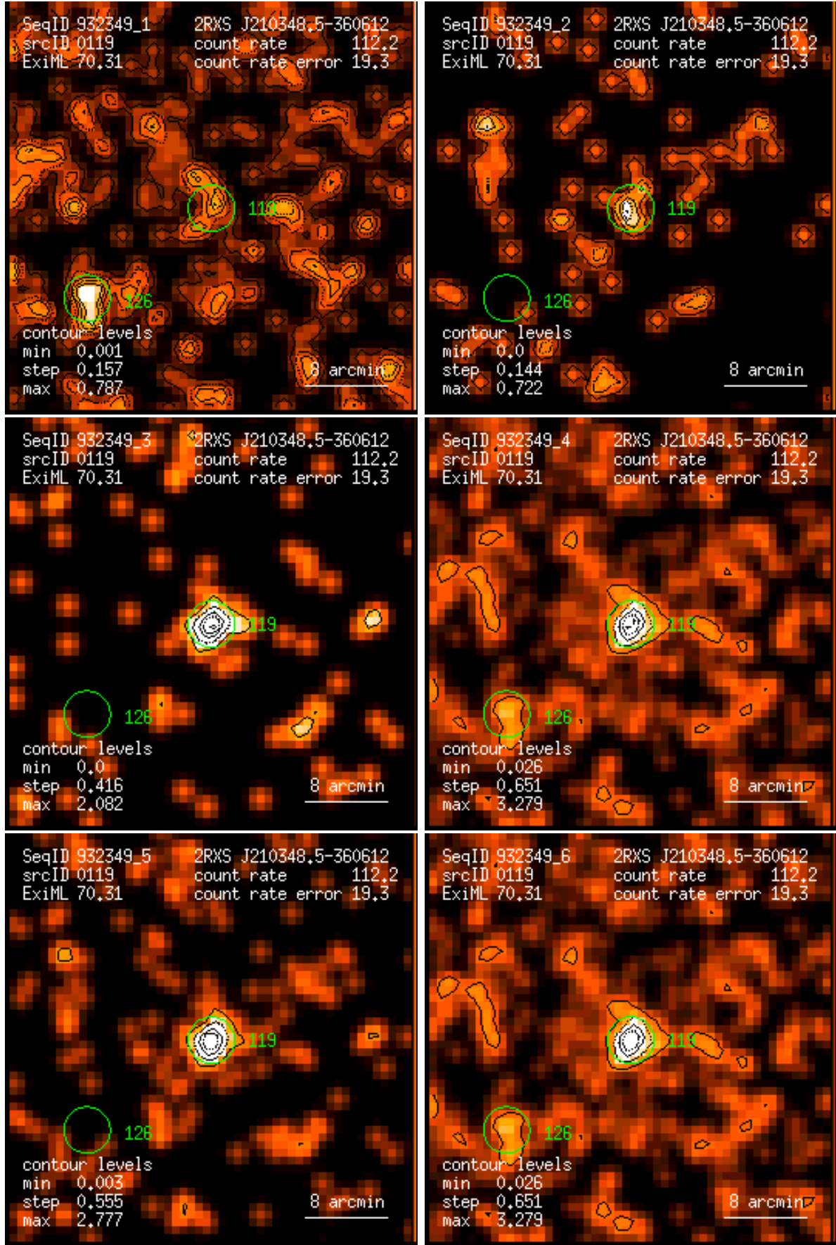
Figure 119: RASS 932349: detection 0119: band rate images, Gaussian filter: (1) PSPC channels 11 – 41, (2) 52 – 90, (3) 91 – 201, (4) 11 – 235, (5) 52 – 201, (6) 11 – 201. Broad band rates in counts/ks. Band rate contour levels in counts/ks/arcmin 2 .
