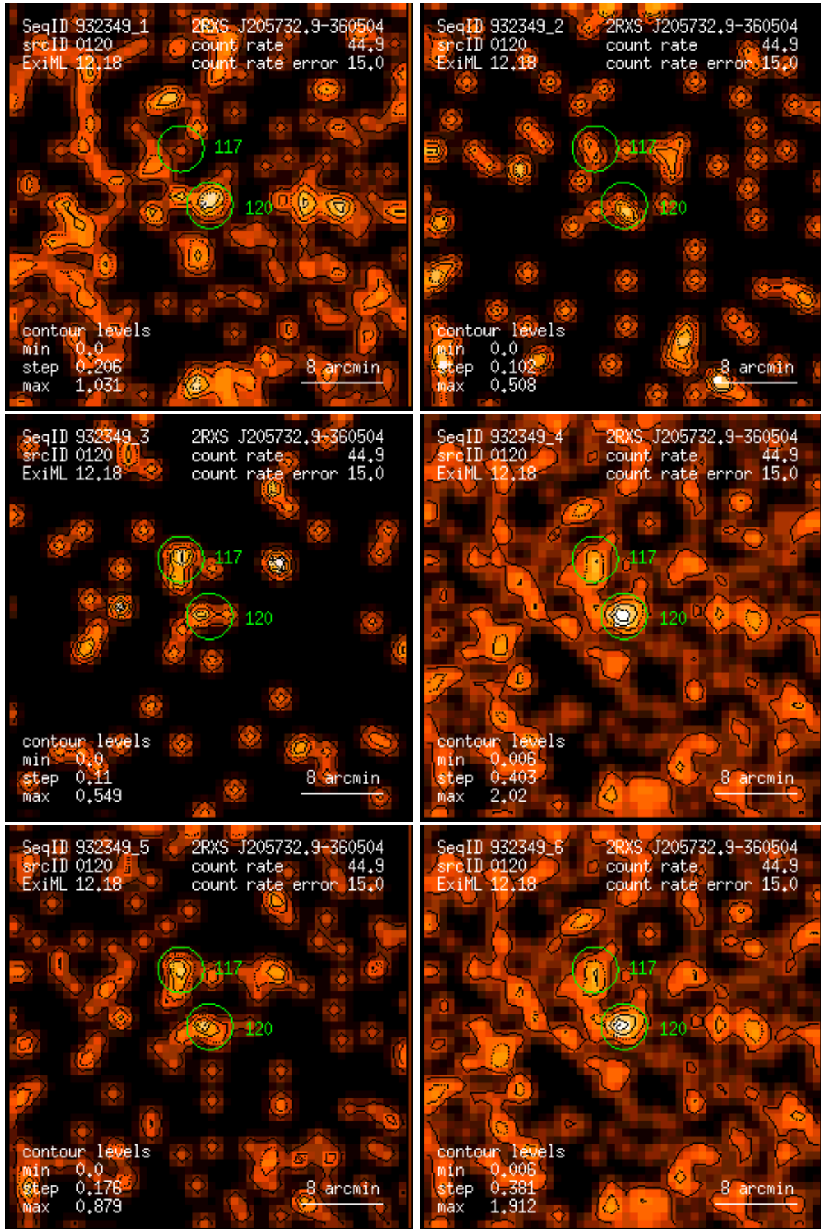
Figure 120: RASS 932349: detection 0120: band rate images, Gaussian filter: (1) PSPC channels 11 – 41, (2) 52 – 90, (3) 91 – 201, (4) 11 – 235, (5) 52 – 201, (6) 11 – 201. Broad band rates in counts/ks. Band rate contour levels in counts/ks/arcmin 2 .
