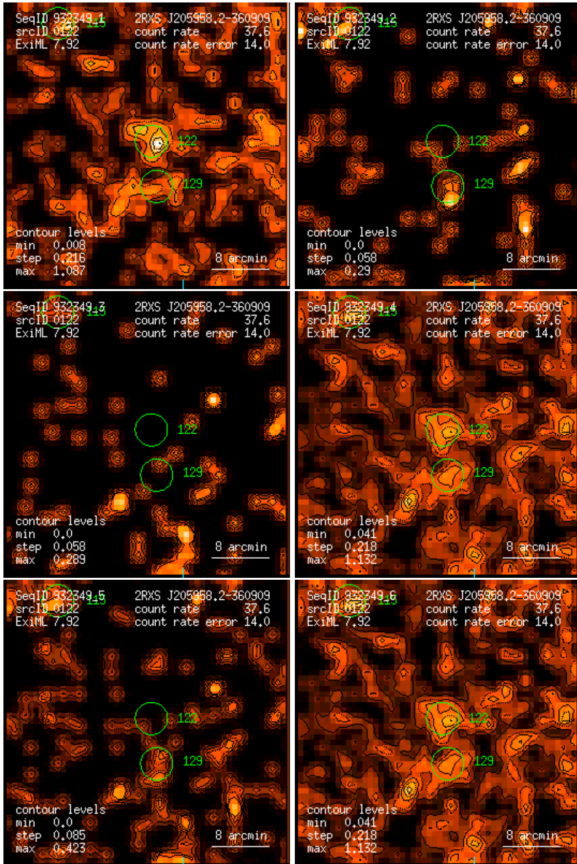
Figure 122: RASS 932349: detection 0122: band rate images, Gaussian filter: (1) PSPC channels 11 – 41, (2) 52 – 90, (3) 91 – 201, (4) 11 – 235, (5) 52 – 201, (6) 11 – 201. Broad band rates in counts/ks. Band rate contour levels in counts/ks/arcmin 2 .
