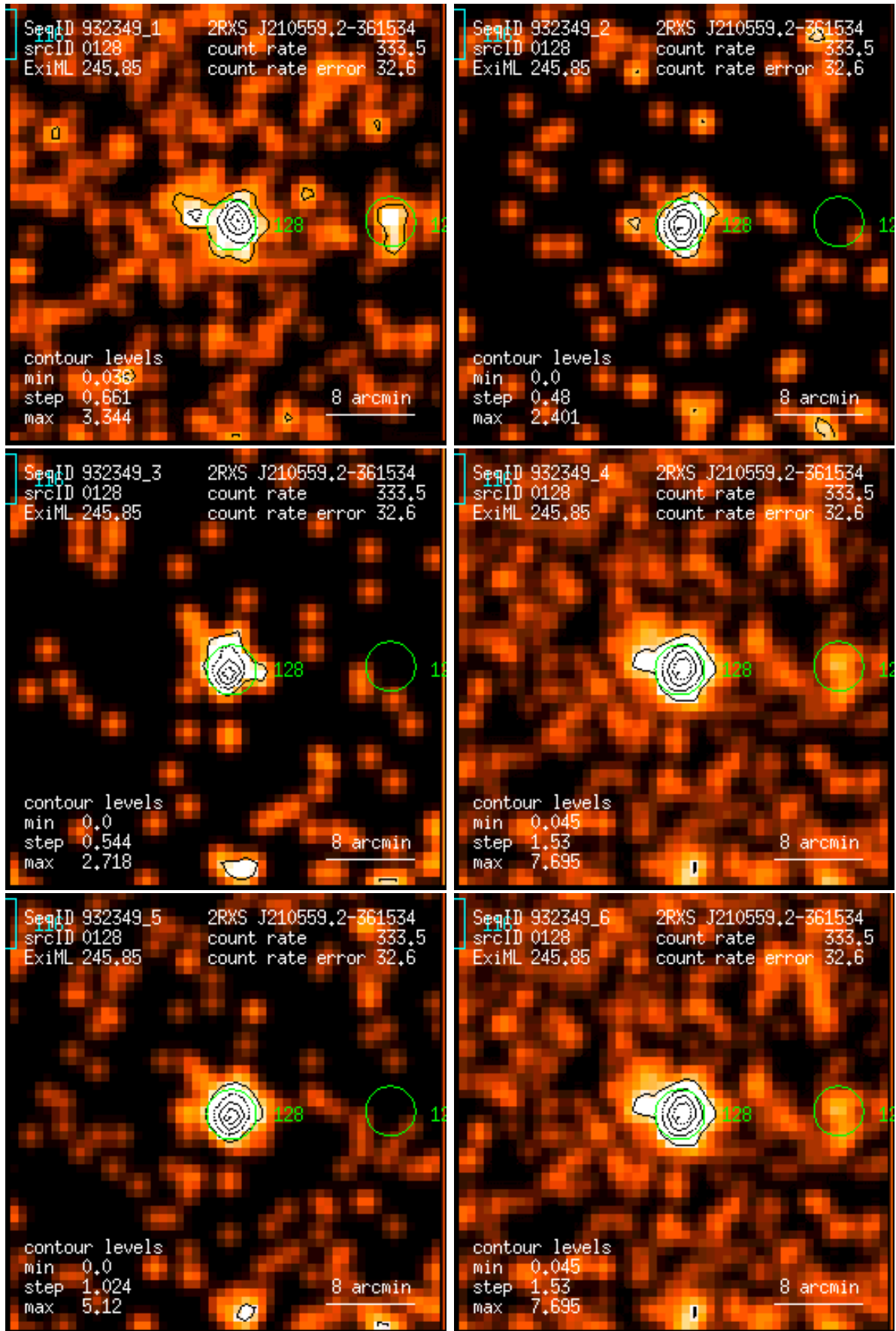
Figure 128: RASS 932349: detection 0128: band rate images, Gaussian filter: (1) PSPC channels 11 – 41, (2) 52 – 90, (3) 91 – 201, (4) 11 – 235, (5) 52 – 201, (6) 11 – 201. Broad band rates in counts/ks. Band rate contour levels in counts/ks/arcmin 2 .
