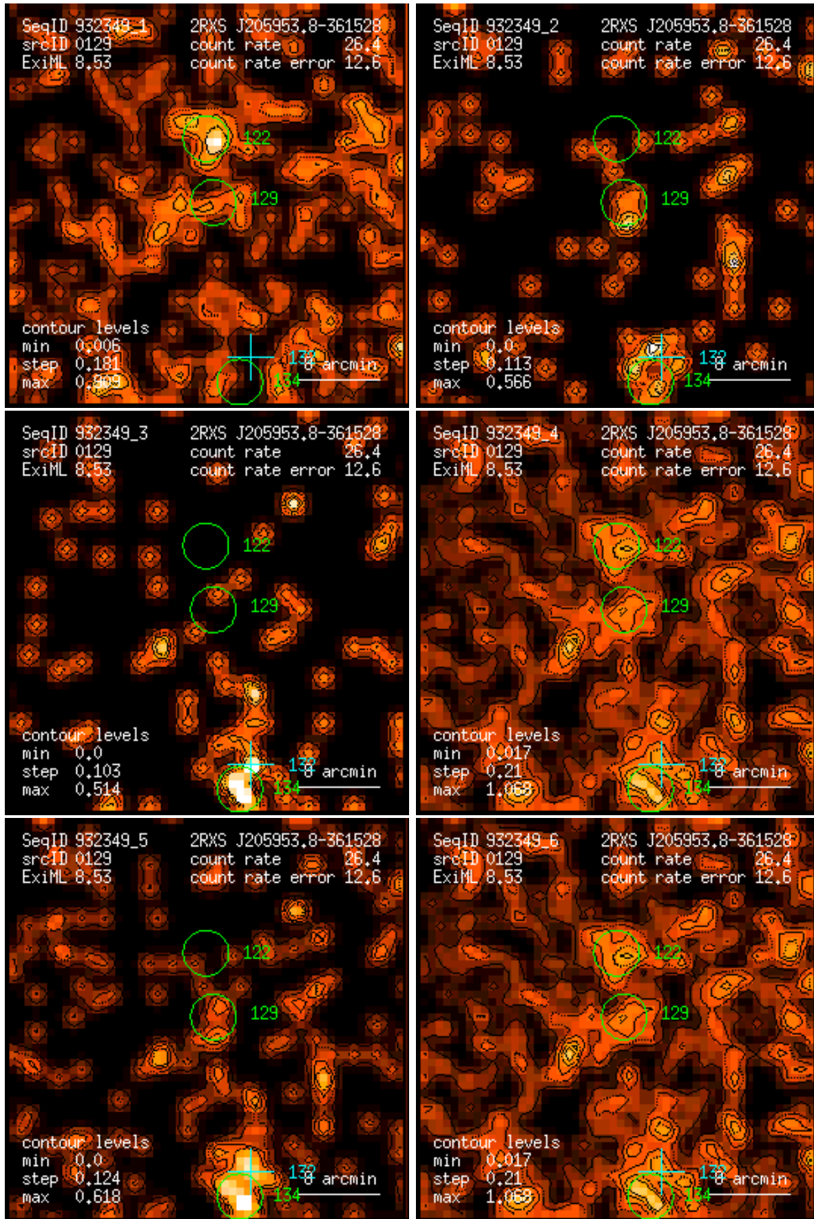
Figure 129: RASS 932349: detection 0129: band rate images, Gaussian filter: (1) PSPC channels 11 – 41, (2) 52 – 90, (3) 91 – 201, (4) 11 – 235, (5) 52 – 201, (6) 11 – 201. Broad band rates in counts/ks. Band rate contour levels in counts/ks/arcmin 2 .
