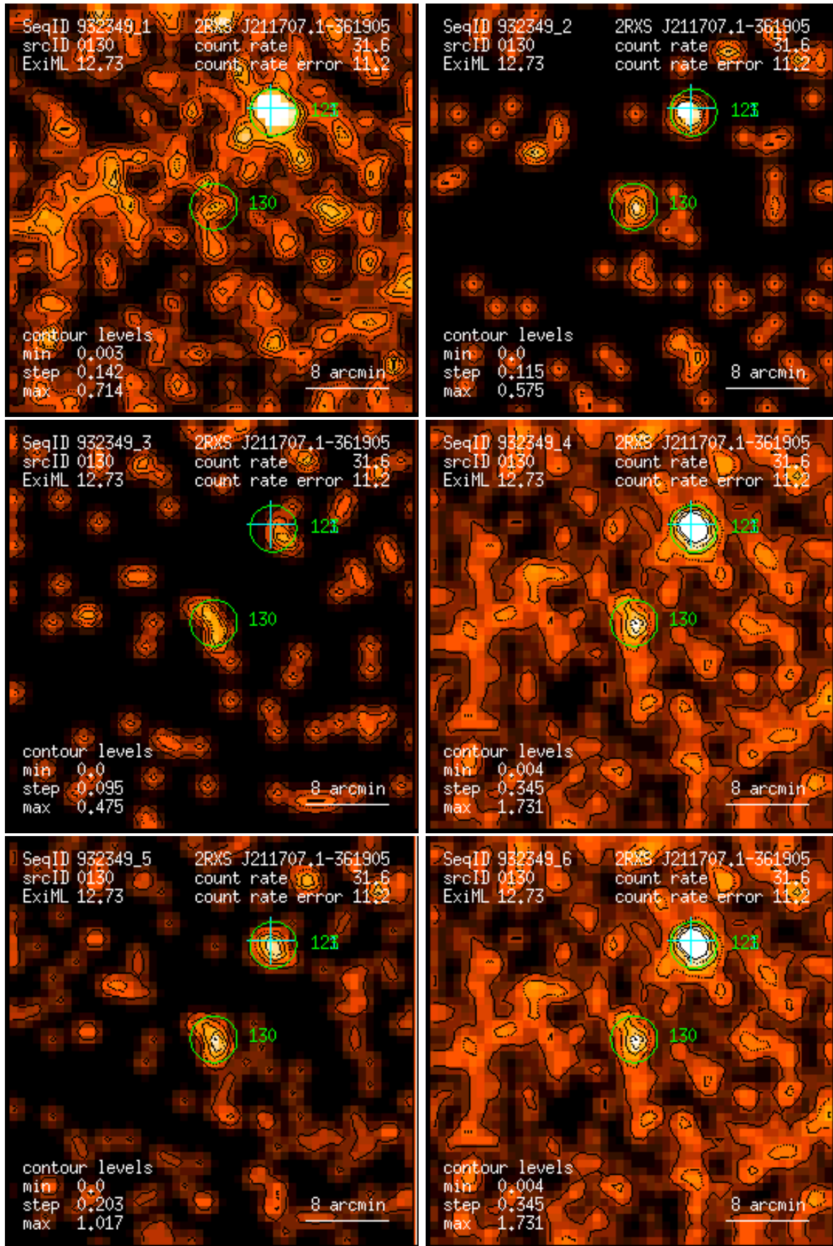
Figure 130: RASS 932349: detection 0130: band rate images, Gaussian filter: (1) PSPC channels 11 – 41, (2) 52 – 90, (3) 91 – 201, (4) 11 – 235, (5) 52 – 201, (6) 11 – 201. Broad band rates in counts/ks. Band rate contour levels in counts/ks/arcmin 2 .
