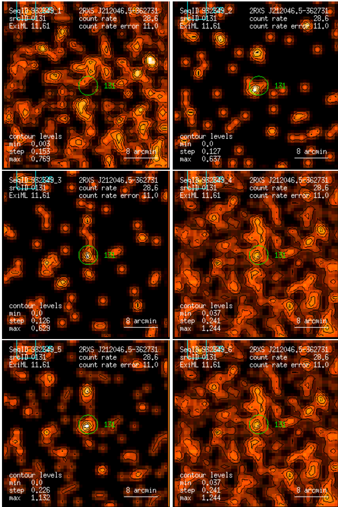
Figure 131: RASS 932349: detection 0131: band rate images, Gaussian filter: (1) PSPC channels 11 – 41, (2) 52 – 90, (3) 91 – 201, (4) 11 – 235, (5) 52 – 201, (6) 11 – 201. Broad band rates in counts/ks. Band rate contour levels in counts/ks/arcmin 2 .
